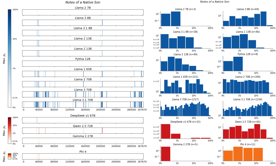
Figure 24: Notes of a Native Son , Baldwin. For 14 LLMs, (left) heatmaps for the sliding-window procedure and (right) corresponding distributions over suffix extraction probabilities ( \tau_{\min} = 0.1\% ).
