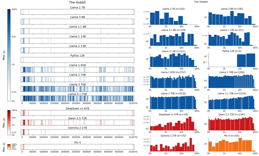
Figure 196: The Hobbit , Tolkien. For 14 LLMs, (left) heatmaps for the sliding-window procedure and (right) corresponding distributions over suffix extraction probabilities ( \tau_{\min} = 0.1\% ).
