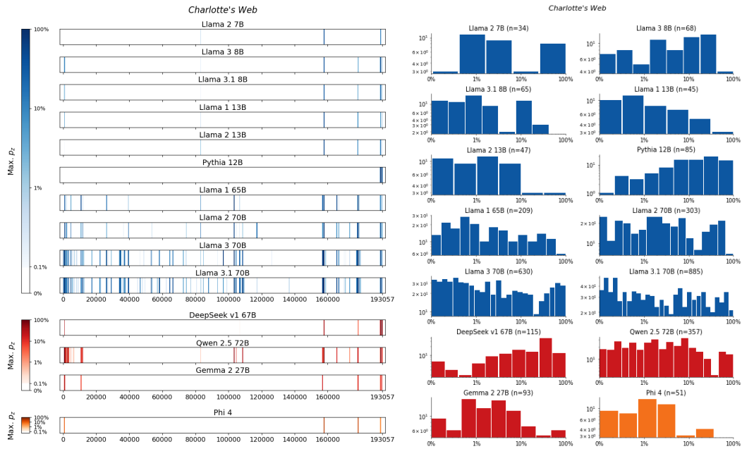
Figure 205: Charlotte's Web , White . For 14 LLMs, (left) heatmaps for the sliding-window procedure and (right) corresponding distributions over suffix extraction probabilities ( \tau_{\min} = 0.1\% ).
