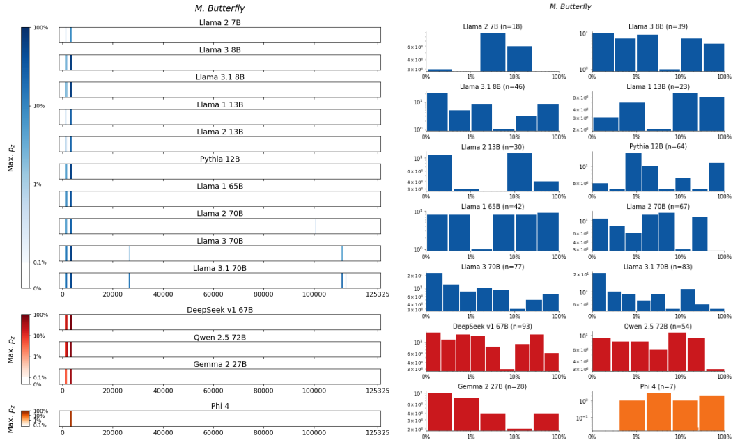
Figure 105: M. Butterfly , Hwang. For 14 LLMs, (left) heatmaps for the sliding-window procedure and (right) corresponding distributions over suffix extraction probabilities ( \tau_{\min} = 0.1\% ).
