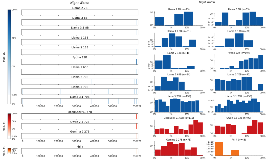
Figure 159: Night Watch, Pratchett . For 14 LLMs, (left) heatmaps for the sliding-window procedure and (right) corresponding distributions over suffix extraction probabilities ( \tau_{\min} = 0.1\% ).
