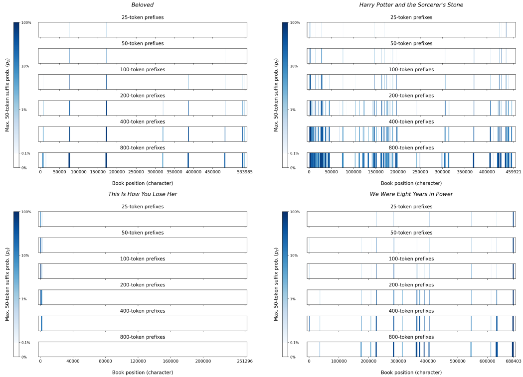
Figure 217: Varying prefix for the LLAMA 3.1 8B baseline. We run the sliding-window procedure for various prefix lengths for 4 books from Books3: Beloved [187], Harry Potter and the Sorcerer’s Stone [224], This Is How You Lose Her [83], and We Were Eight Years in Power [49]. LLAMA models are known to have been trained on Books3. We run probabilistic extraction on LLAMA 3.1 70B with top- k ( T = 1 , k = 40 ) decoding for 50-token suffixes and prefix lengths in \{25, 50, 100, 200, 400, 800\} . Extraction signal generally increases as prefix length increases. However, this only appears to be the case if there is indeed more memorization to surface; increasing prefix length does not always make previously unextractable sequences extractable. There are also diminishing increases as the prefix lengthens.
