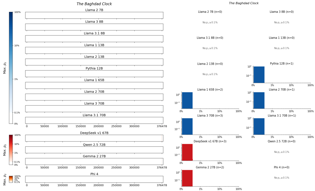
Figure 17: The Baghdad Clock , Al Rawi . For 14 LLMs, (left) heatmaps for the sliding-window procedure and (right) corresponding distributions over suffix extraction probabilities ( \tau_{\min} = 0.1\% ).
