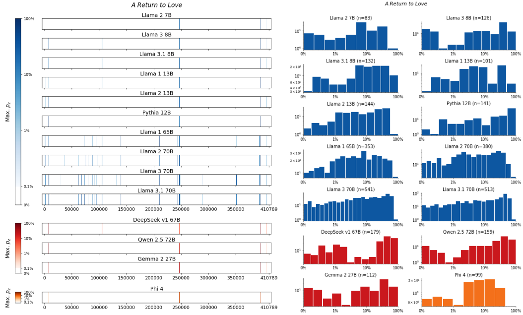
Figure 206: A Return to Love , Williamson . For 14 LLMs, (left) heatmaps for the sliding-window procedure and (right) corresponding distributions over suffix extraction probabilities ( \tau_{\min} = 0.1\% ).
