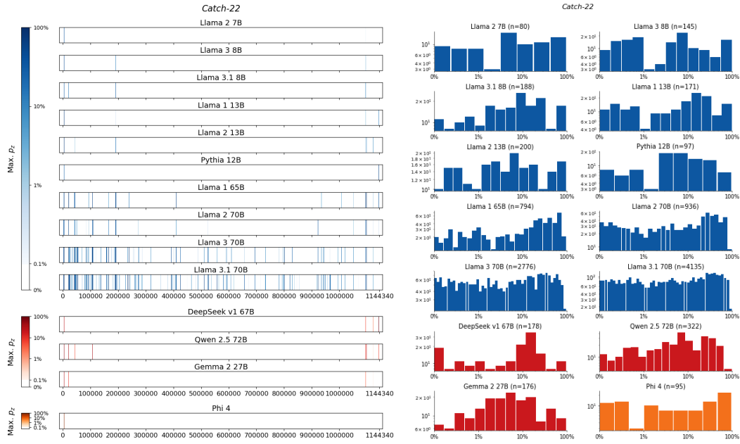
Figure 97: Catch-22 , Heller. For 14 LLMs, (left) heatmaps for the sliding-window procedure and (right) corresponding distributions over suffix extraction probabilities ( \tau_{\min} = 0.1\% ).
