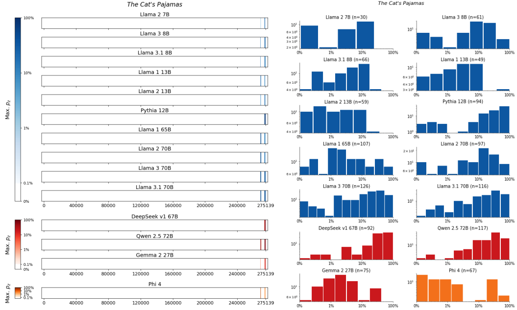
Figure 34: The Cat's Pajamas , Bradbury. For 14 LLMs, (left) heatmaps for the sliding-window procedure and (right) corresponding distributions over suffix extraction probabilities ( \tau_{\min} = 0.1\% ).
