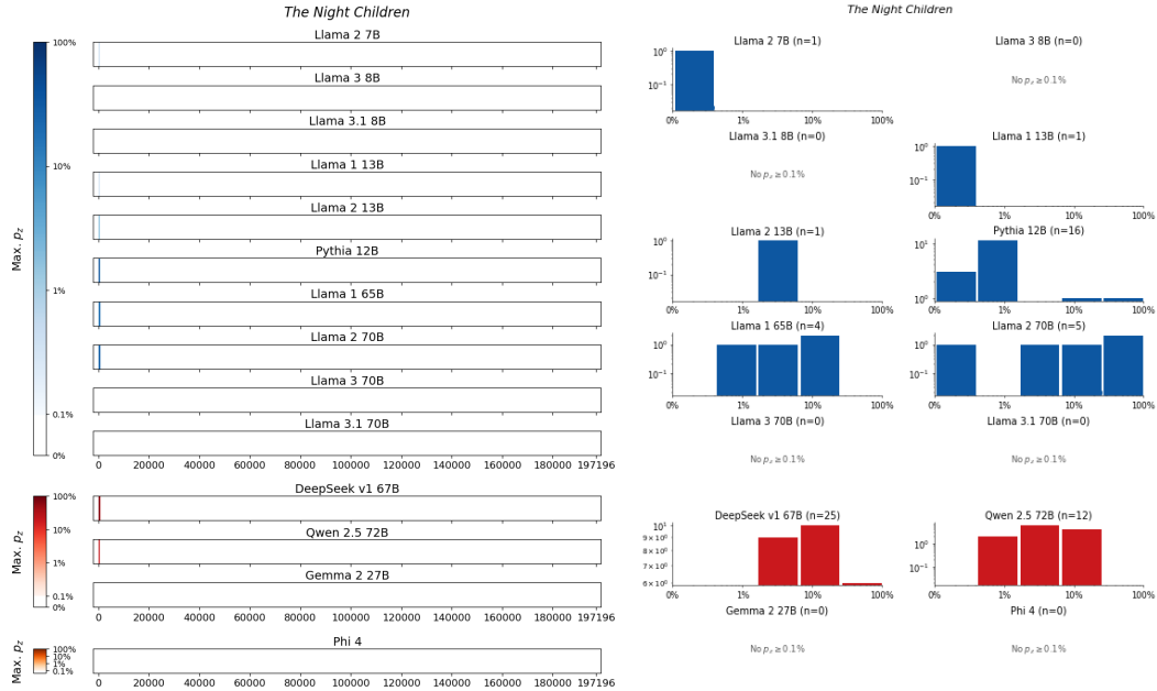
Figure 183: The Night Children, Smith . For 14 LLMs, (left) heatmaps for the sliding-window procedure and (right) corresponding distributions over suffix extraction probabilities ( \tau_{\min} = 0.1\% ).
