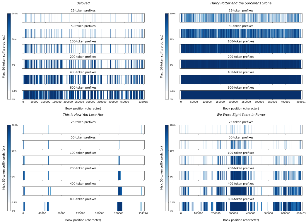
Figure 216: Varying prefix for the LLAMA 3.1 70B baseline. We run the sliding-window procedure for various prefix lengths for 4 books from Books3: Beloved [187], Harry Potter and the Sorcerer’s Stone [224], This Is How You Lose Her [83], and We Were Eight Years in Power [49]. LLAMA models are known to have been trained on Books3. We run probabilistic extraction on LLAMA 3.1 70B with top- k ( T = 1 , k = 40 ) decoding for 50-token suffixes and prefix lengths in \{25, 50, 100, 200, 400, 800\} . Extraction signal generally increases as prefix length increases. However, this only appears to be the case if there is indeed more memorization to surface; increasing prefix length does not always make previously unextractable sequences extractable. There are also diminishing increases as the prefix lengthens.
