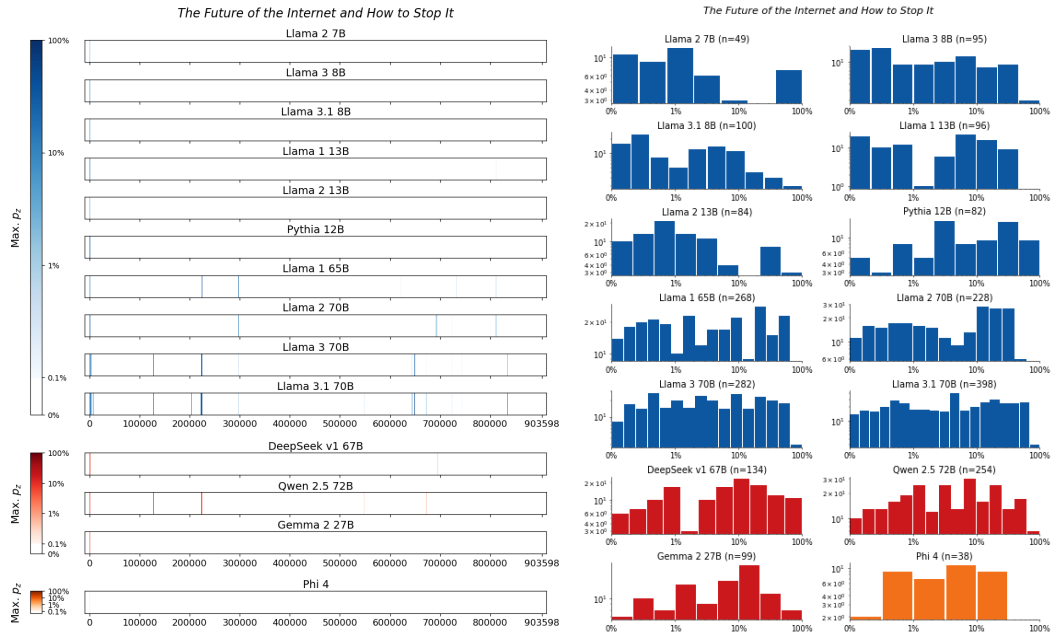
Figure 212: The Future of the Internet and How to Stop It , Zittrain . For 14 LLMs, (left) heatmaps for the sliding-window procedure and (right) corresponding distributions over suffix extraction probabilities ( \tau_{\min} = 0.1\% ).
