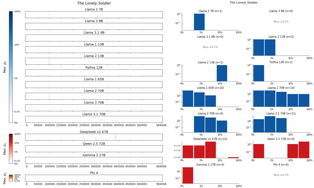
Figure 31: The Lonely Soldier , Benedict . For 14 LLMs, (left) heatmaps for the sliding-window procedure and (right) corresponding distributions over suffix extraction probabilities ( \tau_{\min} = 0.1\% ).
