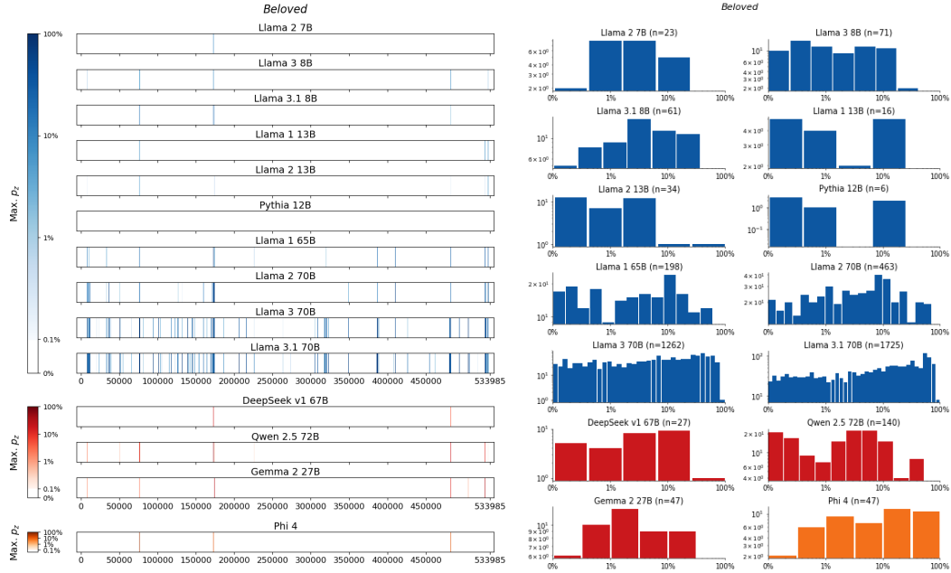
Figure 141: Beloved , Morrison . For 14 LLMs, (left) heatmaps for the sliding-window procedure and (right) corresponding distributions over suffix extraction probabilities ( \tau_{\min} = 0.1\% ).
