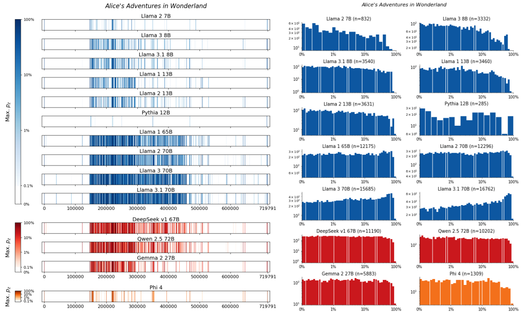
Figure 41: Alice's Adventures in Wonderland , Carroll. For 14 LLMs, (left) heatmaps for the sliding-window procedure and (right) corresponding distributions over suffix extraction probabilities ( \tau_{\min} = 0.1\% ).
