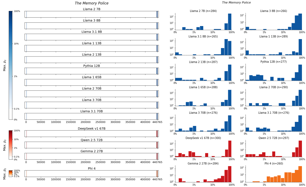
Figure 147: The Memory Police , Ogawa. For 14 LLMs, (left) heatmaps for the sliding-window procedure and (right) corresponding distributions over suffix extraction probabilities ( \tau_{\min} = 0.1\% ).
