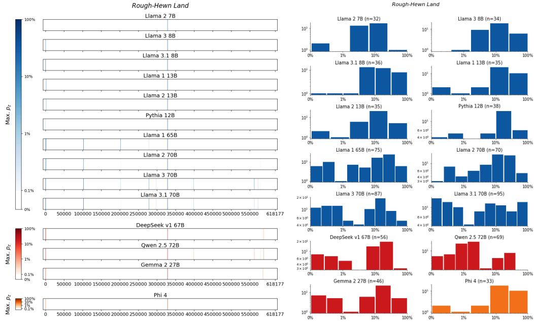
Figure 131: Rough-Hewn Land, Meldahl . For 14 LLMs, (left) heatmaps for the sliding-window procedure and (right) corresponding distributions over suffix extraction probabilities ( \tau_{\min} = 0.1\% ).
