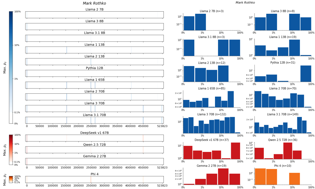
Figure 51: Mark Rothko , Cohen-Solal. For 14 LLMs, (left) heatmaps for the sliding-window procedure and (right) corresponding distributions over suffix extraction probabilities ( \tau_{\min} = 0.1\% ).
