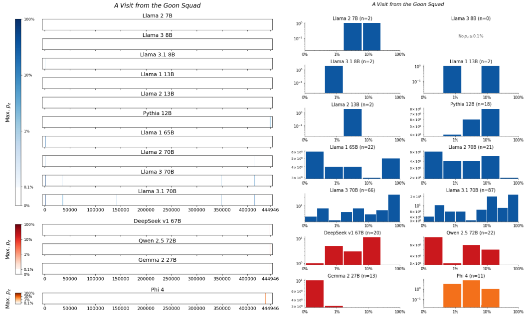
Figure 69: A Visit from the Goon Squad, Egan . For 14 LLMs, (left) heatmaps for the sliding-window procedure and (right) corresponding distributions over suffix extraction probabilities ( \tau_{\min} = 0.1\% ).
