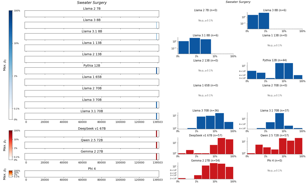
Figure 80: Sweater Surgery , Girard. For 14 LLMs, (left) heatmaps for the sliding-window procedure and (right) corresponding distributions over suffix extraction probabilities ( \tau_{\min} = 0.1\% ).
