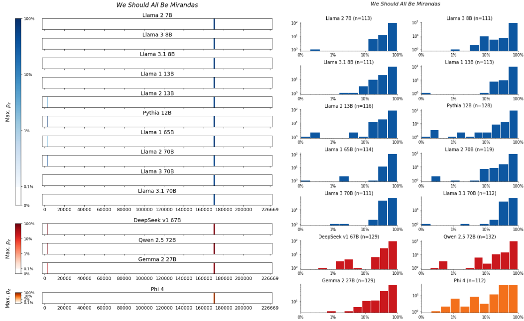
Figure 71: We Should All Be Mirandas , Fairless and Garroni. For 14 LLMs, (left) heatmaps for the sliding-window procedure and (right) corresponding distributions over suffix extraction probabilities ( \tau_{\min} = 0.1\% ).
