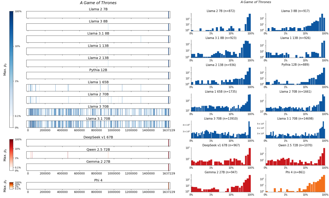
Figure 130: A Game of Thrones, Martin . For 14 LLMs, (left) heatmaps for the sliding-window procedure and (right) corresponding distributions over suffix extraction probabilities ( \tau_{\min} = 0.1\% ).
