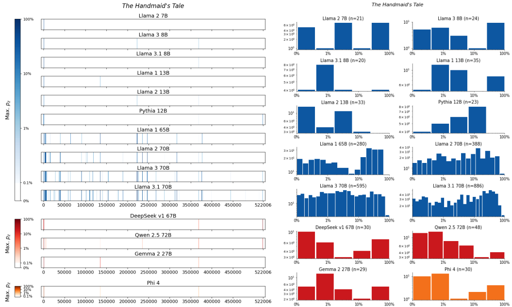
Figure 21: The Handmaid's Tale , Atwood. For 14 LLMs, (left) heatmaps for the sliding-window procedure and (right) corresponding distributions over suffix extraction probabilities ( \tau_{\min} = 0.1\% ).
