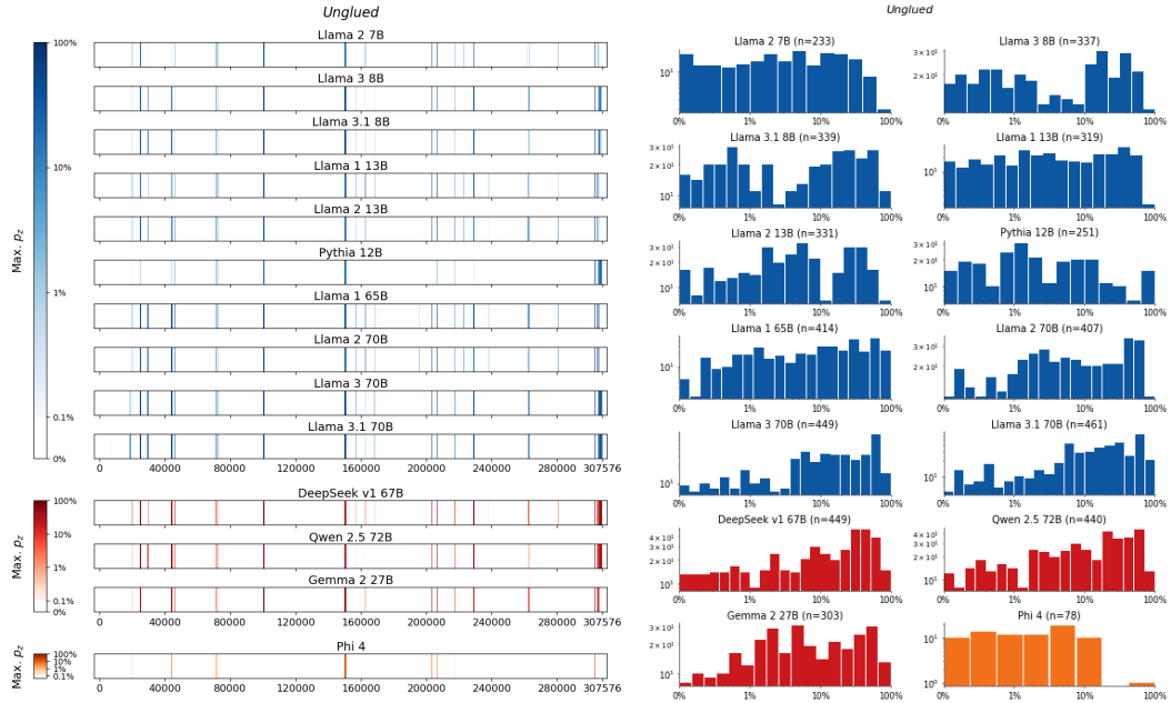
Figure 193: Unglued , TerKeurst . For 14 LLMs, (left) heatmaps for the sliding-window procedure and (right) corresponding distributions over suffix extraction probabilities ( \tau_{\min} = 0.1\% ).
