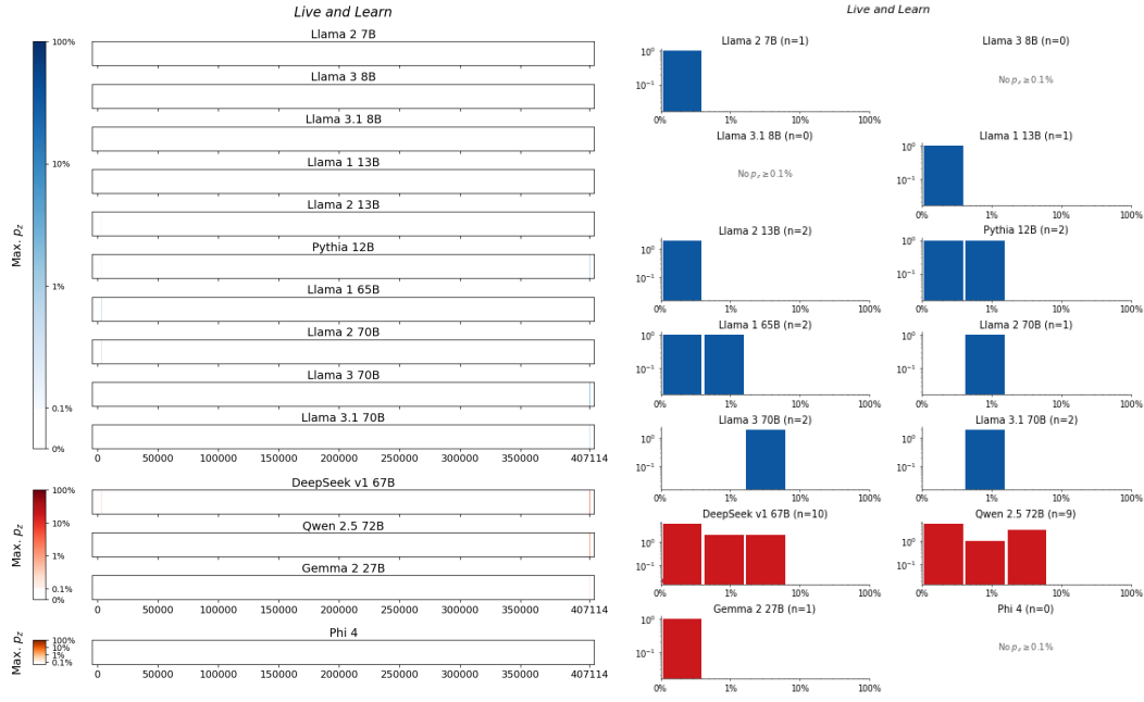
Figure 38: Live and Learn , Bryant. For 14 LLMs, (left) heatmaps for the sliding-window procedure and (right) corresponding distributions over suffix extraction probabilities ( \tau_{\min} = 0.1\% ).
