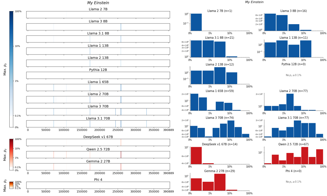
Figure 36: My Einstein , Brockman . For 14 LLMs, (left) heatmaps for the sliding-window procedure and (right) corresponding distributions over suffix extraction probabilities ( \tau_{\min} = 0.1\% ).
