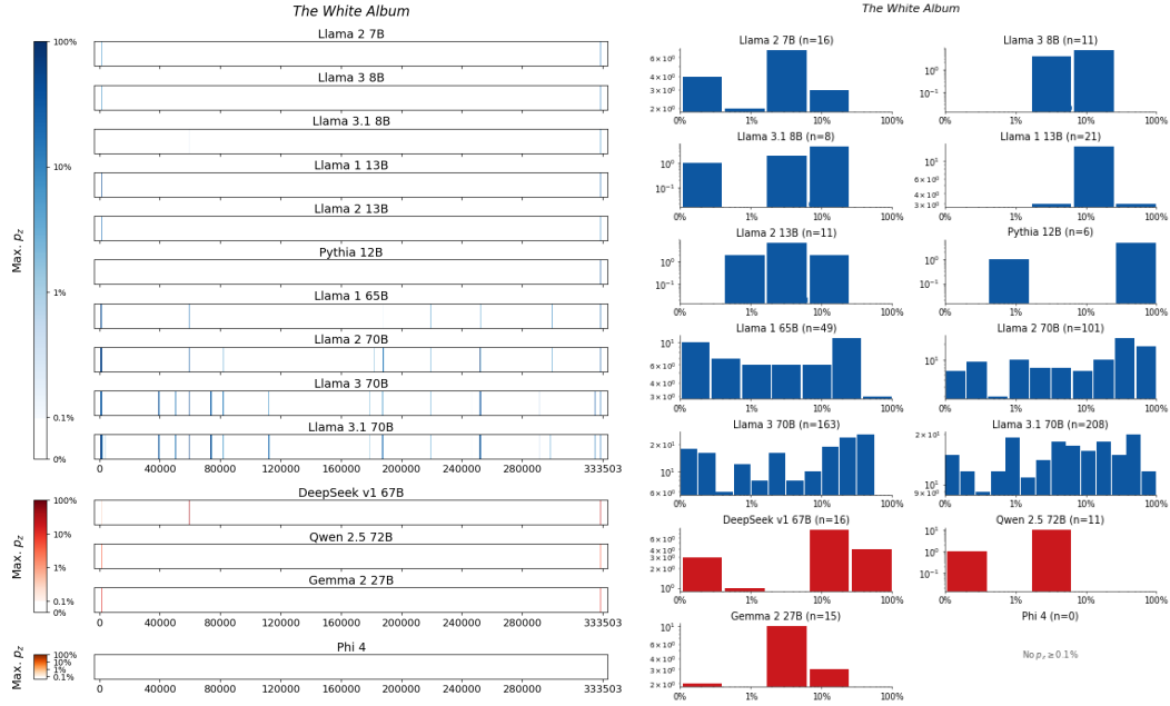
Figure 66: The White Album, Didion . For 14 LLMs, (left) heatmaps for the sliding-window procedure and (right) corresponding distributions over suffix extraction probabilities ( \tau_{\min} = 0.1\% ).
