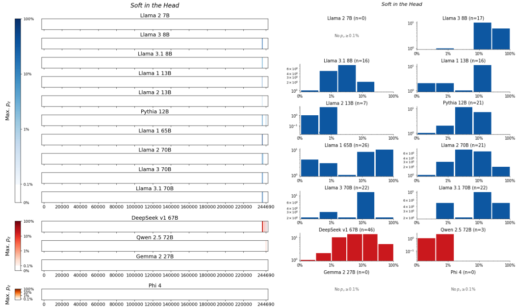
Figure 164: Soft in the Head, Roger . For 14 LLMs, (left) heatmaps for the sliding-window procedure and (right) corresponding distributions over suffix extraction probabilities ( \tau_{\min} = 0.1\% ).
