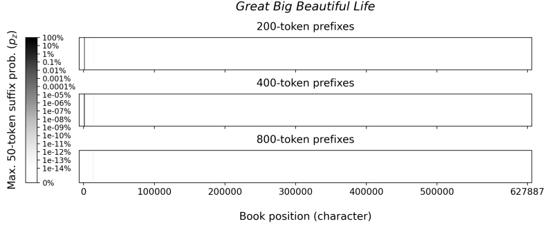
Figure 221: Chance generation of non-training data. We show LLAMA 3.1 70B and top- k ( T=1 , k=40 ) decoding on Great Big Beautiful Life [128] (published spring 2025), with respect to 50-token suffixes and prefix lengths in \{200, 400, 800\} tokens. Except for the copyright notice at the beginning, we do not register any p_z \geq \tau_{\min} = 0.1\% . We register no other suffix probabilities p_z \geq 10^{-13}\% , and only 1 (out of \sim 62,000 sequences) for which p_z \geq 10^{-14}\% . (See the faint gray band near 20K characters.)
