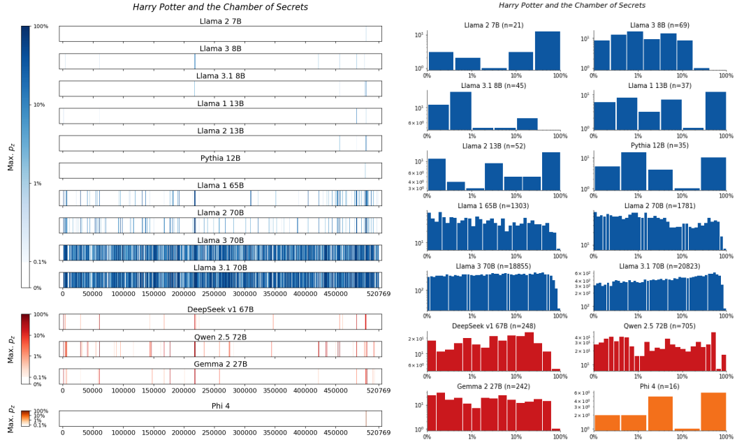
Figure 167: Harry Potter and the Chamber of Secrets , Rowling. For 14 LLMs, (left) heatmaps for the sliding-window procedure and (right) corresponding distributions over suffix extraction probabilities ( \tau_{\min} = 0.1\% ).
