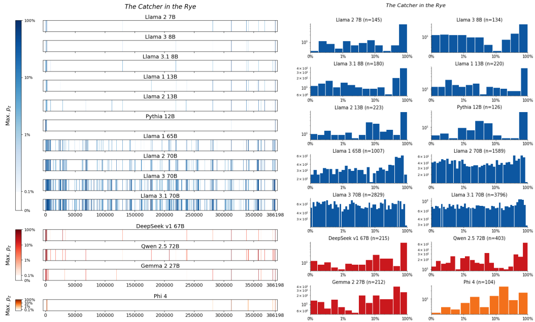
Figure 175: The Catcher in the Rye , Salinger. For 14 LLMs, (left) heatmaps for the sliding-window procedure and (right) corresponding distributions over suffix extraction probabilities ( \tau_{\min} = 0.1\% ).
