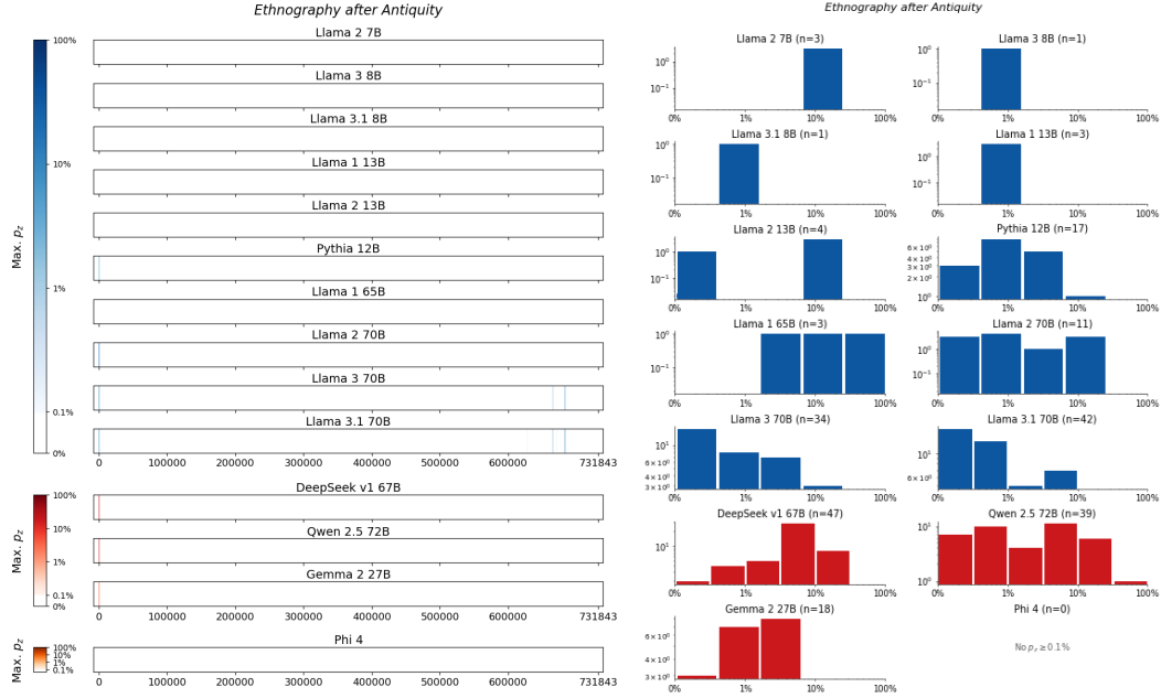
Figure 112: Ethnography after Antiquity , Kaldellis. For 14 LLMs, (left) heatmaps for the sliding-window procedure and (right) corresponding distributions over suffix extraction probabilities ( \tau_{\min} = 0.1\% ).
