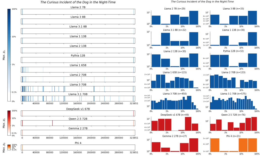
Figure 92: The Curious Incident of the Dog in the Night-Time , Haddon. For 14 LLMs, (left) heatmaps for the sliding-window procedure and (right) corresponding distributions over suffix extraction probabilities ( \tau_{\min} = 0.1\% ).
