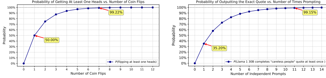
Figure 12: Probability of an event occurring at least once changes as a function of n independent trials. Following the intuition of flipping a fair coin (where heads has p_z = 0.5 = 50\% ), we show how the probability of flipping heads at least once changes with more flips ( left ). We show how the probability p of generating the verbatim suffix of the “careless people” quote at least once for LLAMA 1 30B ( p_z \approx 35.2\% ) changes as a function of the number of independent prompts to the model with the prefix ( right ). Both figures use 1 - (1 - p_z)^n (Equation 6), plugging in the respective p_z (for the coin flip and for generating the “careless people” suffix given the prefix) and different values of n to compute p .
