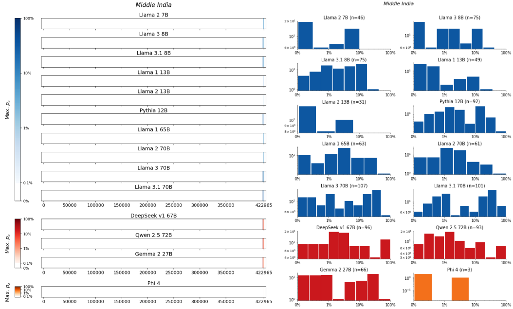
Figure 174: Middle India , Sahni. For 14 LLMs, (left) heatmaps for the sliding-window procedure and (right) corresponding distributions over suffix extraction probabilities ( \tau_{\min} = 0.1\% ).
