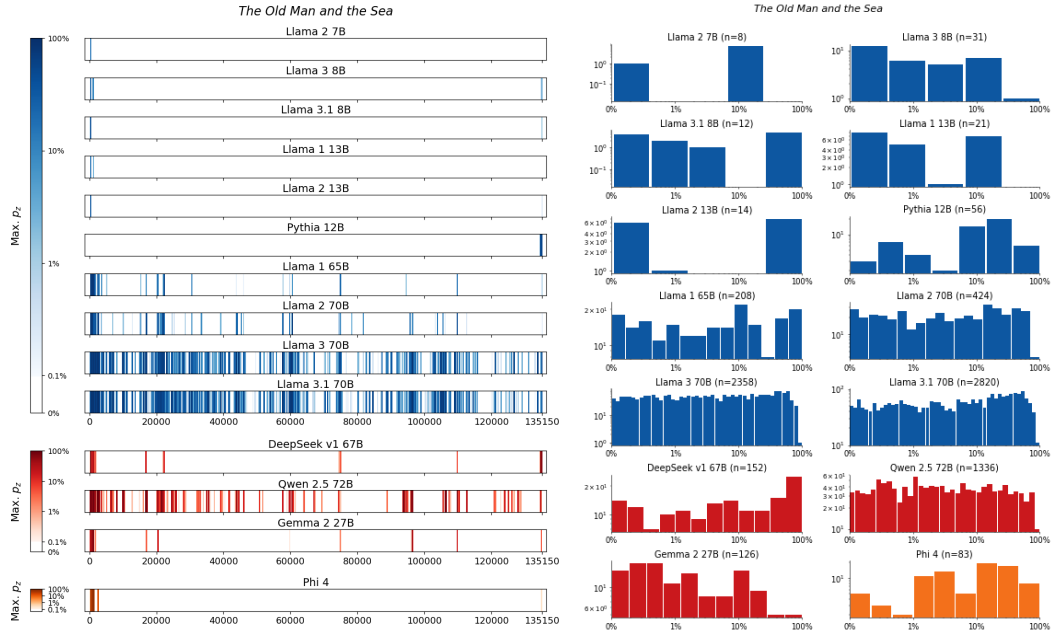
Figure 98: The Old Man and the Sea , Hemingway. For 14 LLMs, (left) heatmaps for the sliding-window procedure and (right) corresponding distributions over suffix extraction probabilities ( \tau_{\min} = 0.1\% ).
