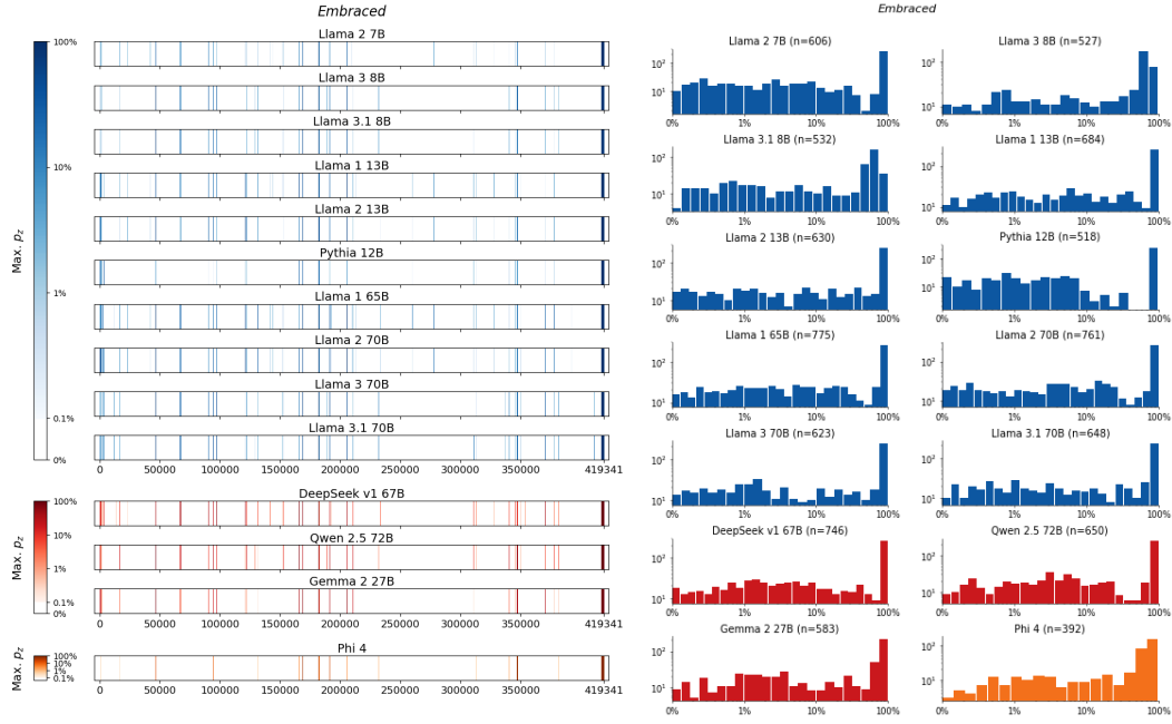
Figure 194: Embraced , TerKeurst . For 14 LLMs, (left) heatmaps for the sliding-window procedure and (right) corresponding distributions over suffix extraction probabilities ( \tau_{\min} = 0.1\% ).
