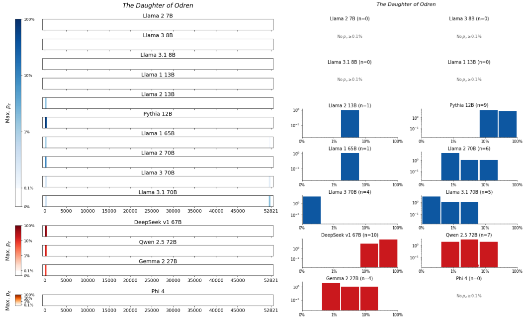
Figure 122: The Daughter of Odren, Le Guin . For 14 LLMs, (left) heatmaps for the sliding-window procedure and (right) corresponding distributions over suffix extraction probabilities ( \tau_{\min} = 0.1\% ).
