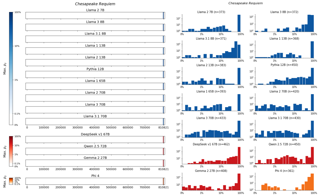
Figure 191: Chesapeake Requiem , Swift . For 14 LLMs, (left) heatmaps for the sliding-window procedure and (right) corresponding distributions over suffix extraction probabilities ( \tau_{\min} = 0.1\% ).
