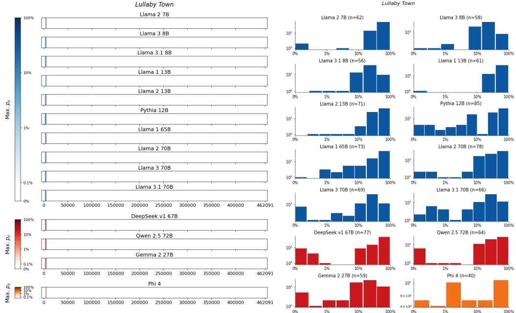
Figure 56: Lullaby Town, Crais . For 14 LLMs, (left) heatmaps for the sliding-window procedure and (right) corresponding distributions over suffix extraction probabilities ( \tau_{\min} = 0.1\% ).
