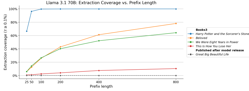
Figure 215: Extraction coverage by prefix length. Plotting extraction coverage for \tau = \tau_{\min} = 0.1\% (Equation 10) for the 5 books we test with varying prefix lengths and LLAMA 3.1 70B. Four of these books are in Books3 and thus in LLAMA’s training data. The remaining book, Great Big Beautiful Life , is used in our negative controls on non-training data; extraction coverage is 0% regardless of prefix length. As we increase prefix length, extraction coverage for each book in the training data begins to level off. While Harry Potter and the Sorcerer’s Stone is entirely memorized by the model, it does not appear to be the case that Beloved , We Were Eight Years in Power , or This Is How You Lose Her would be entirely extractable with respect to 50-token suffixes and even longer prefixes.
