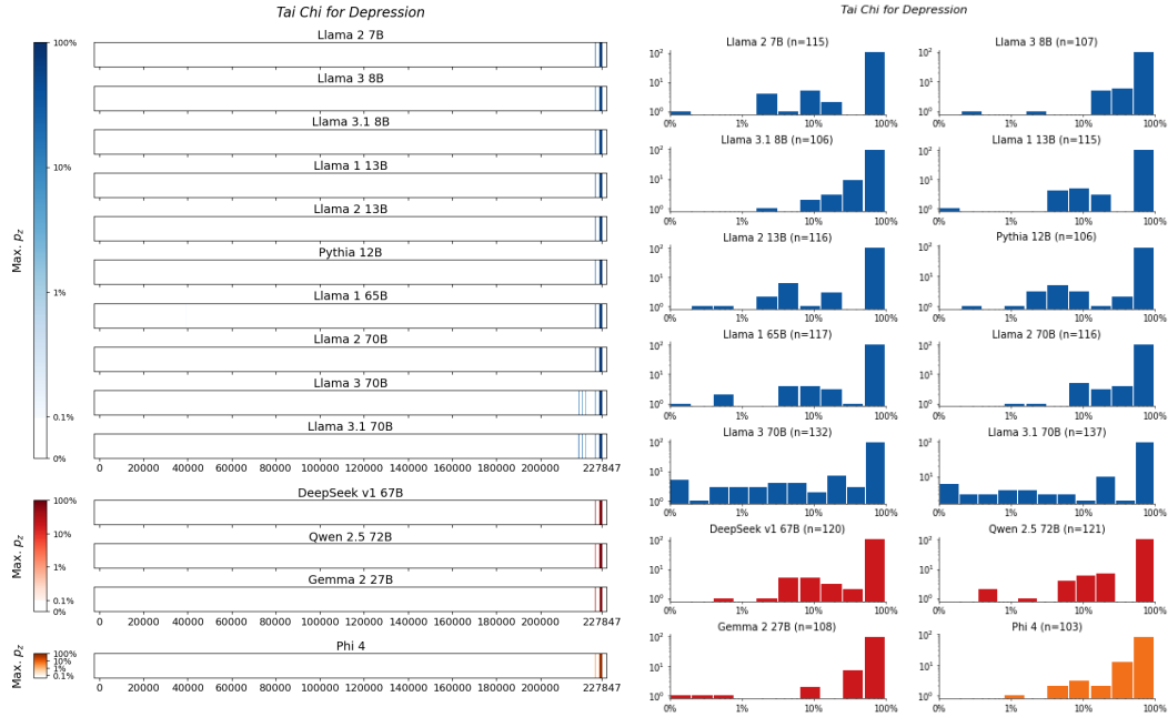
Figure 115: Tai Chi for Depression , Kuhn. For 14 LLMs, (left) heatmaps for the sliding-window procedure and (right) corresponding distributions over suffix extraction probabilities ( \tau_{\min} = 0.1\% ).
