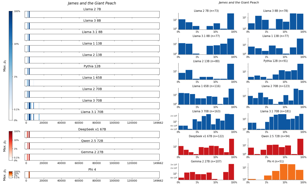
Figure 61: James and the Giant Peach , Dahl. For 14 LLMs, (left) heatmaps for the sliding-window procedure and (right) corresponding distributions over suffix extraction probabilities ( \tau_{\min} = 0.1\% ).
