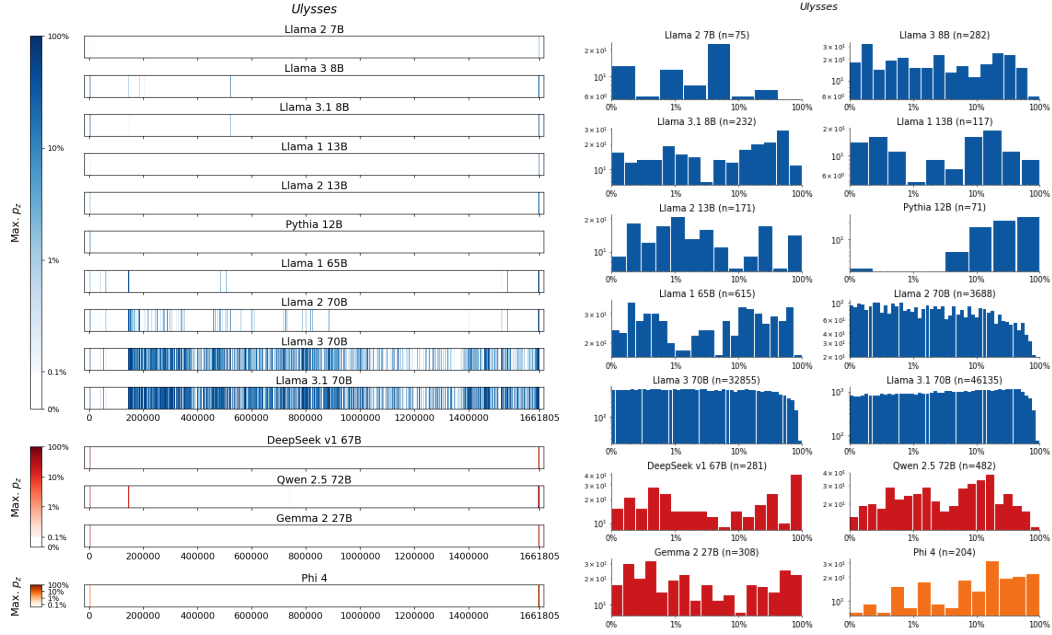
Figure 110: Ulysses, Joyce . For 14 LLMs, (left) heatmaps for the sliding-window procedure and (right) corresponding distributions over suffix extraction probabilities ( \tau_{\min} = 0.1\% ).
