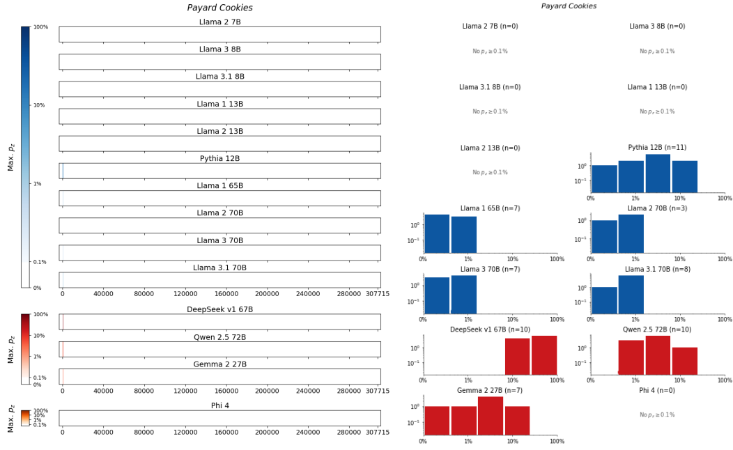
Figure 154: Payard Cookies , Payard and McBride. For 14 LLMs, (left) heatmaps for the sliding-window procedure and (right) corresponding distributions over suffix extraction probabilities ( \tau_{\min} = 0.1\% ).
