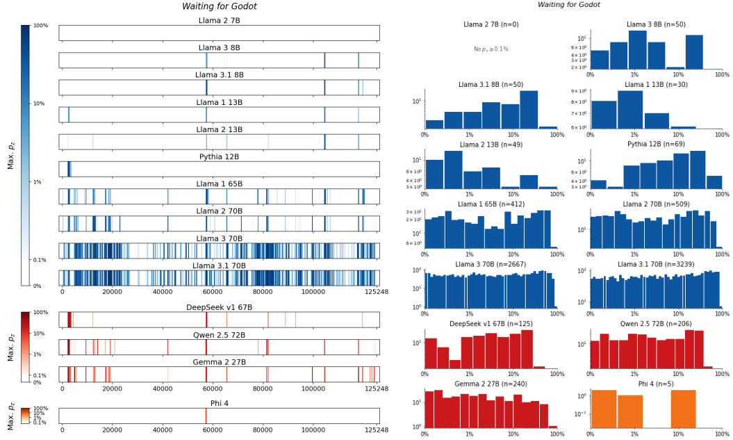
Figure 30: Waiting for Godot , Beckett . For 14 LLMs, (left) heatmaps for the sliding-window procedure and (right) corresponding distributions over suffix extraction probabilities ( \tau_{\min} = 0.1\% ).
