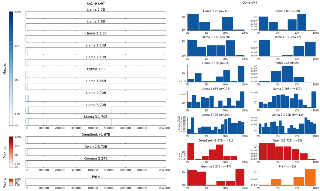
Figure 75: Gone Girl , Flynn . For 14 LLMs, (left) heatmaps for the sliding-window procedure and (right) corresponding distributions over suffix extraction probabilities ( \tau_{\min} = 0.1\% ).
