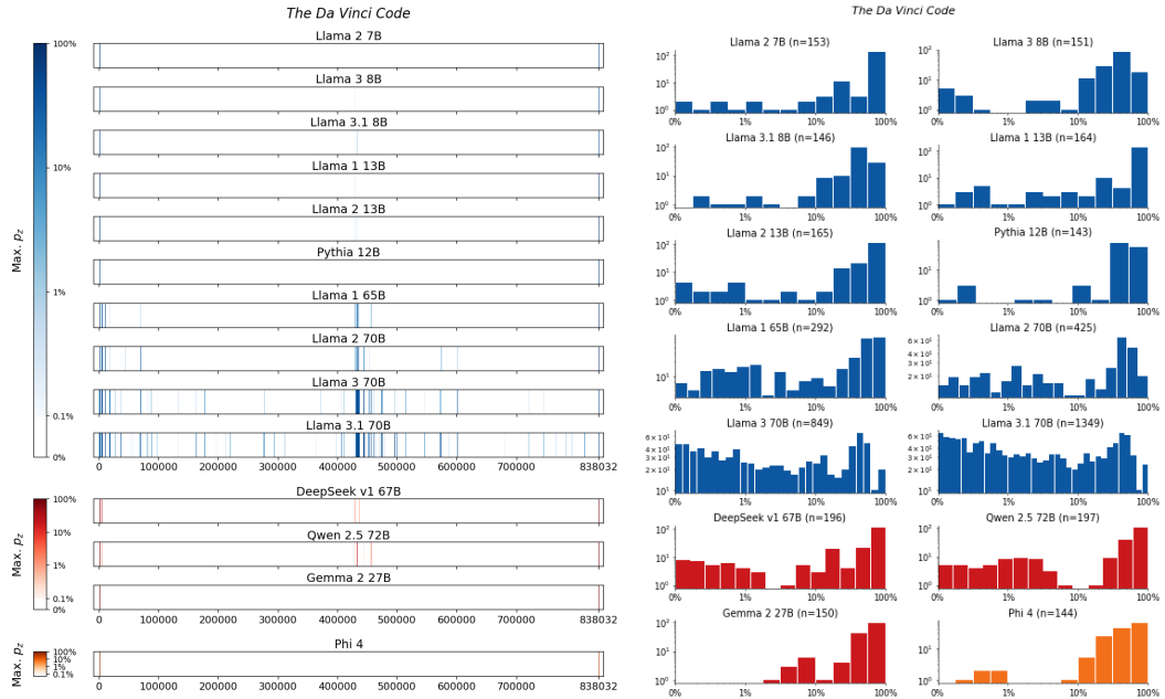
Figure 37: The Da Vinci Code , Brown . For 14 LLMs, (left) heatmaps for the sliding-window procedure and (right) corresponding distributions over suffix extraction probabilities ( \tau_{\min} = 0.1\% ).
