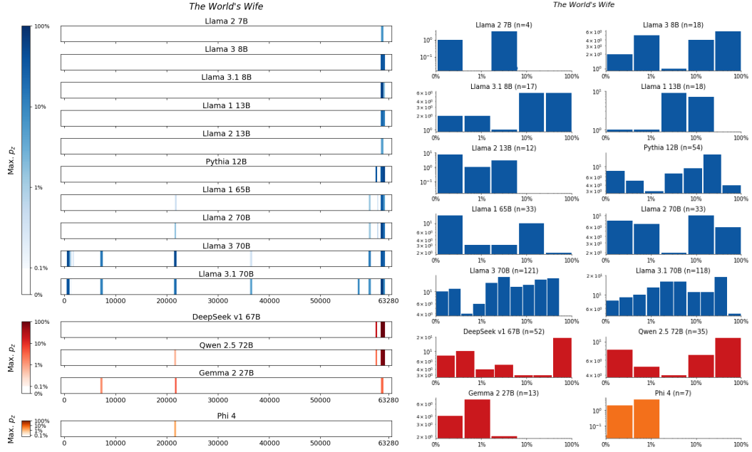
Figure 68: The World's Wife, Duffy . For 14 LLMs, (left) heatmaps for the sliding-window procedure and (right) corresponding distributions over suffix extraction probabilities ( \tau_{\min} = 0.1\% ).
