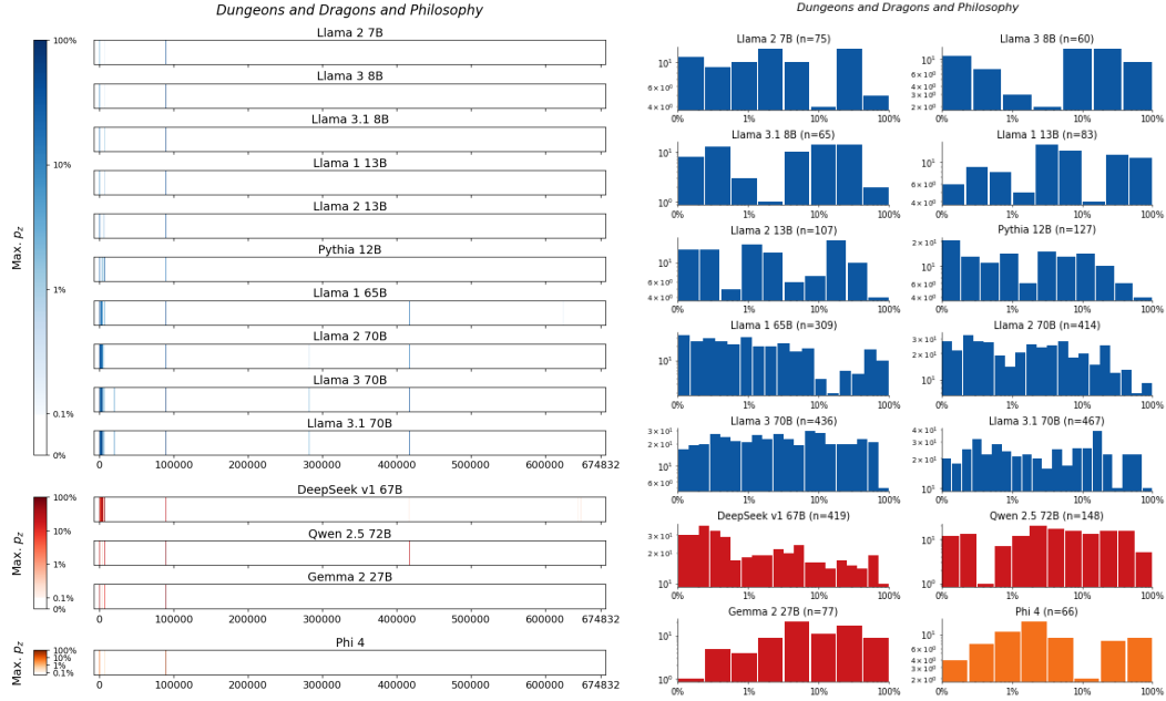
Figure 50: Dungeons and Dragons and Philosophy , Cogburn and Silcox. For 14 LLMs, (left) heatmaps for the sliding-window procedure and (right) corresponding distributions over suffix extraction probabilities ( \tau_{\min} = 0.1\% ).
