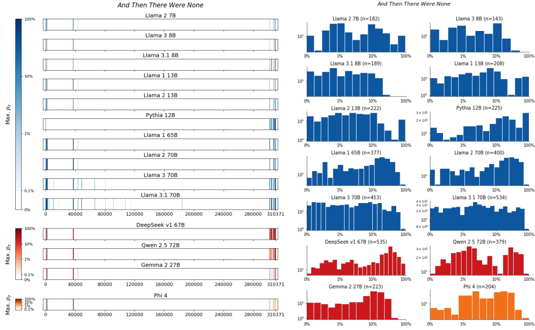
Figure 44: And Then There Were None, Christie . For 14 LLMs, (left) heatmaps for the sliding-window procedure and (right) corresponding distributions over suffix extraction probabilities ( \tau_{\min} = 0.1\% ).
