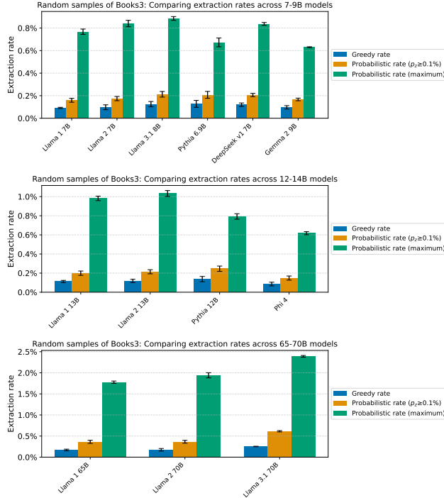
Figure 13: Extended extraction rate results. Comparing greedy discoverable and probabilistic extraction rates (for a our conservative setting, p_z \geq \tau_{\min} = 0.1\% ). As a reference point, we also include the maximum possible rate of generating 50-token sequences that match our suffixes drawn from Books3 for small (7–9B), medium (12–14B), and large models (65–70B). (This is akin to looking at all p_z > 0 .) Probabilistic rates are computed with top- k sampling using T = 1 and k = 40 . The maximum probabilistic rate should be understood as a very loose upper bound on extraction of memorized training data; it also captures generalization. Average extraction rates (i.e., \tau_{\min} = 0.1\% ) on randomly sampled Books3 sequences are relatively low for all models. Aligning with prior work, we observe that larger models memorize more. For our setting, this is true for both within and across model families. PHI 4, a 14B model, is an exception: its extraction rates are on par with smaller models. Error bars here indicate variance across the 3 samples of 40,000 sequences that we run.
