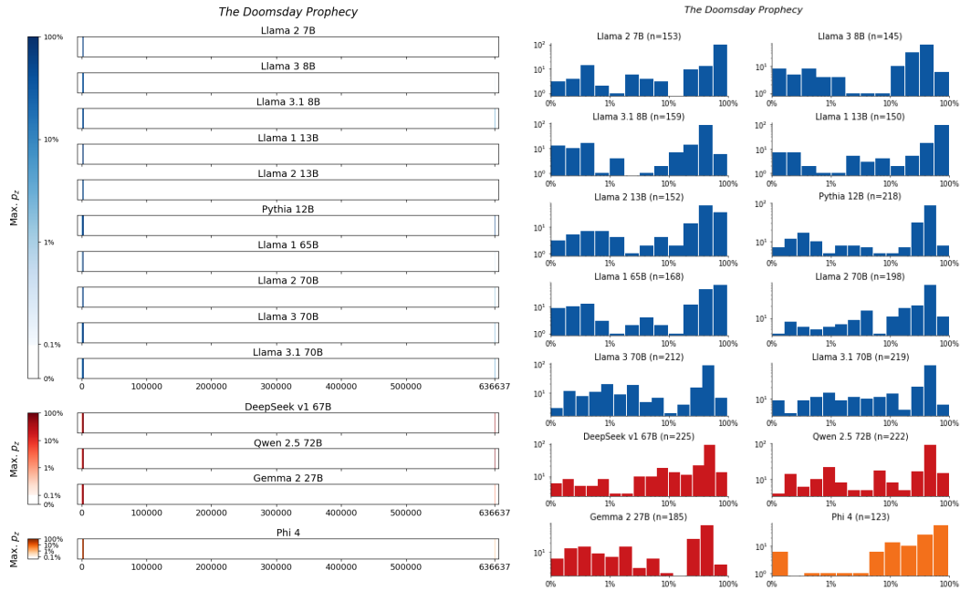
Figure 129: The Domsday Prophecy , Mariani. For 14 LLMs, (left) heatmaps for the sliding-window procedure and (right) corresponding distributions over suffix extraction probabilities ( \tau_{\min} = 0.1\% ).
