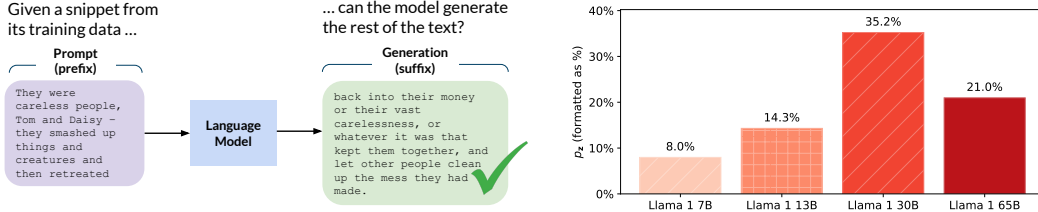
Figure 1: Quantifying memorization for a sequence drawn from The Great Gatsby . (left) Discoverable extraction [41, 157] prompts an LLM with a training-data prefix, and checks if the resulting generation exactly matches the ground-truth suffix. (right) Probabilistic extraction [123] measures the probability p_z (%) of generating the exact suffix given the prefix, shown here for LLAMA 1 models on the same quote from The Great Gatsby . LLAMA 1 30B exhibits the highest extraction risk.
