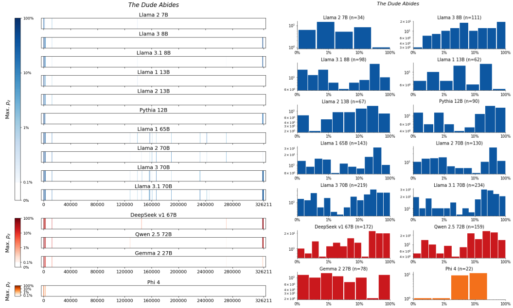
Figure 72: The Dude Abides , Falsani . For 14 LLMs, (left) heatmaps for the sliding-window procedure and (right) corresponding distributions over suffix extraction probabilities ( \tau_{\min} = 0.1\% ).
