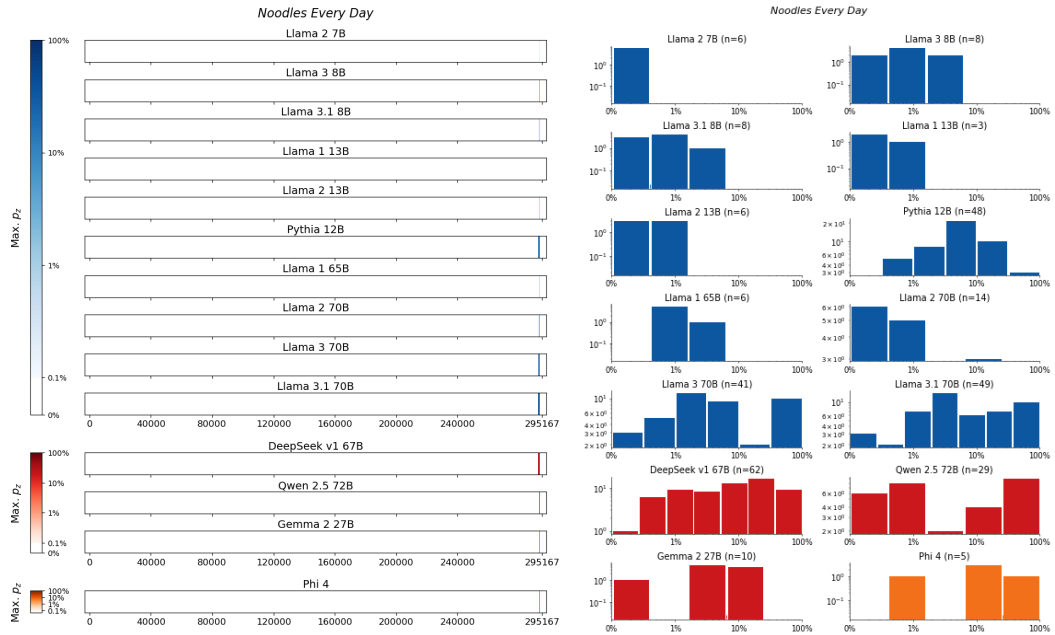
Figure 199: Noodles Every Day , Trang . For 14 LLMs, (left) heatmaps for the sliding-window procedure and (right) corresponding distributions over suffix extraction probabilities ( \tau_{\min} = 0.1\% ).
