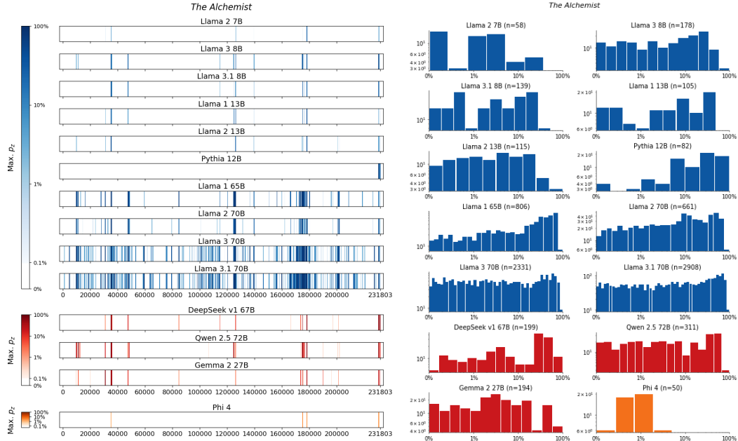
Figure 49: The Alchemist, Coelho . For 14 LLMs, (left) heatmaps for the sliding-window procedure and (right) corresponding distributions over suffix extraction probabilities ( \tau_{\min} = 0.1\% ).
