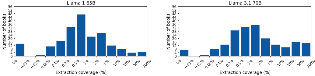
Figure 4: LLM-specific distributions over extraction coverage. Extraction coverage (Equation 4) differs across LLMs for the 200 books we evaluate, illustrated for LLAMA 1 65B and LLAMA 3.1 70B. Results use 100-token sequences (50-token prefix + 50-token suffix), top- k decoding ( T=1 , k=40 ), and \tau_{\min}=0.1\% as the coverage threshold \tau .
