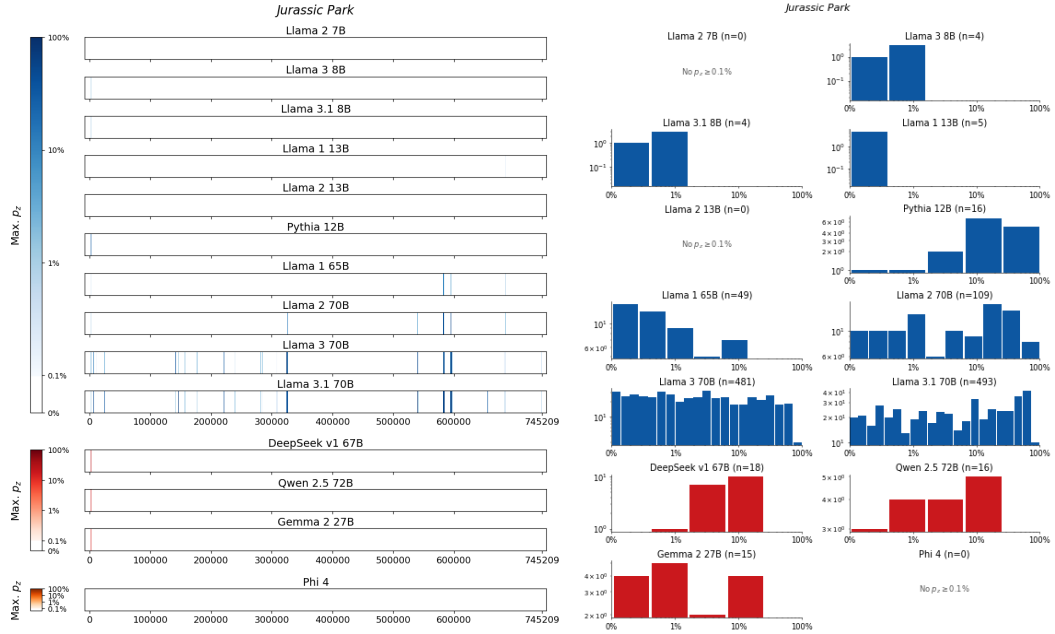
Figure 57: Jurassic Park, Crichton . For 14 LLMs, (left) heatmaps for the sliding-window procedure and (right) corresponding distributions over suffix extraction probabilities ( \tau_{\min} = 0.1\% ).
