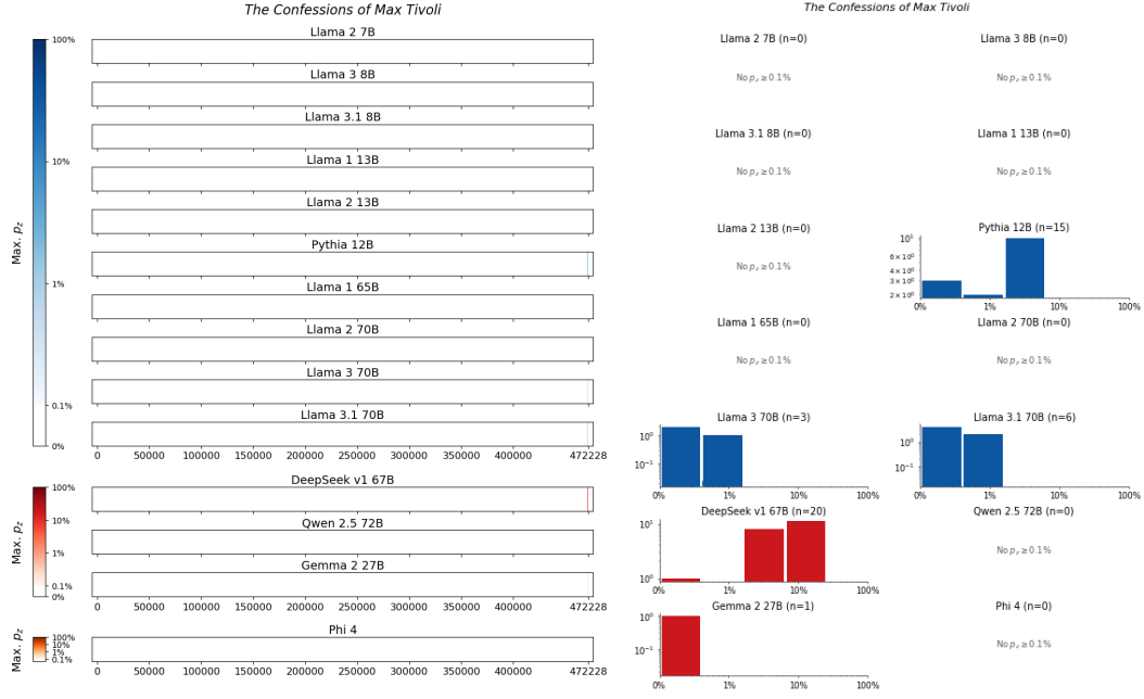
Figure 90: The Confessions of Max Tivoli , Greer. For 14 LLMs, (left) heatmaps for the sliding-window procedure and (right) corresponding distributions over suffix extraction probabilities ( \tau_{\min} = 0.1\% ).
