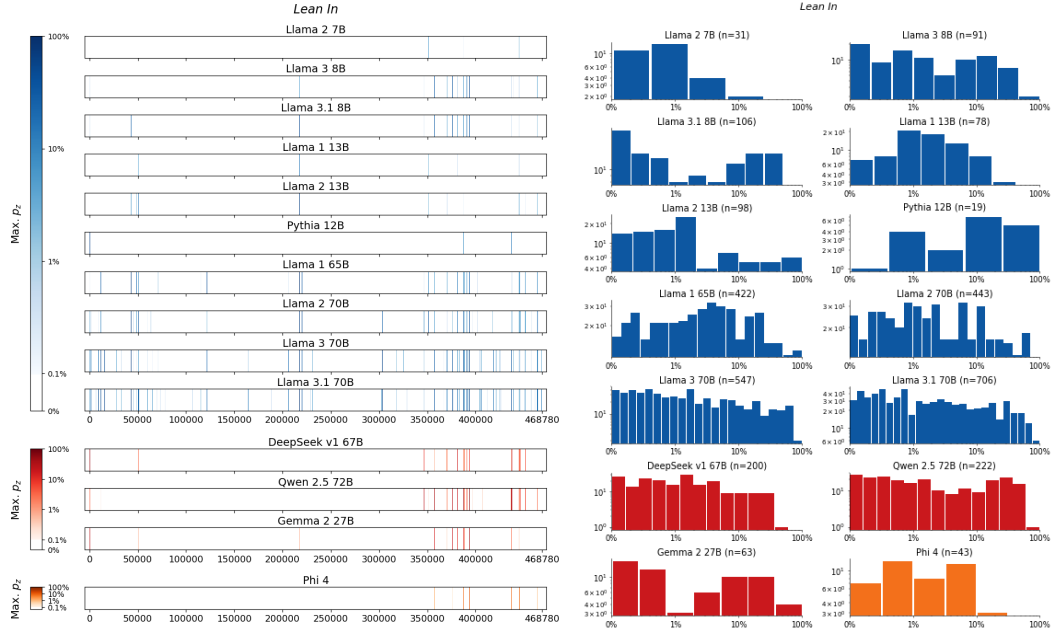
Figure 176: Lean In , Sandberg. For 14 LLMs, (left) heatmaps for the sliding-window procedure and (right) corresponding distributions over suffix extraction probabilities ( \tau_{\min} = 0.1\% ).
