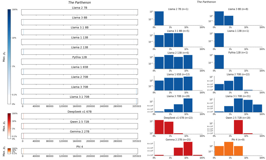
Figure 28: The Parthenon, Beard . For 14 LLMs, (left) heatmaps for the sliding-window procedure and (right) corresponding distributions over suffix extraction probabilities ( \tau_{\min} = 0.1\% ).
