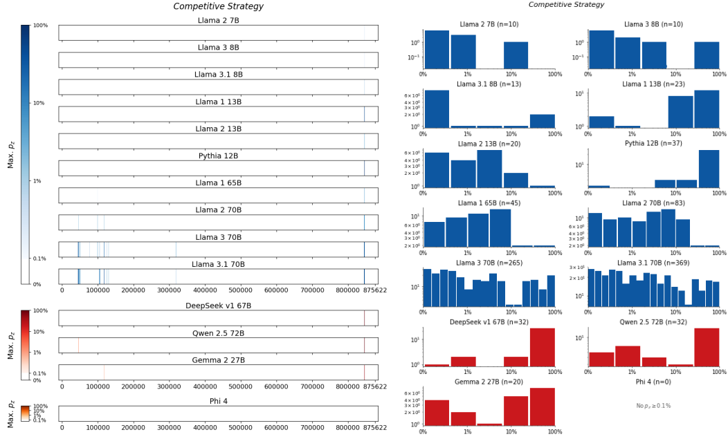
Figure 158: Competitive Strategy, Porter . For 14 LLMs, (left) heatmaps for the sliding-window procedure and (right) corresponding distributions over suffix extraction probabilities ( \tau_{\min} = 0.1\% ).
