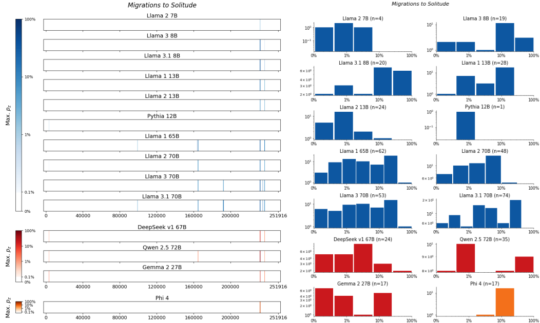
Figure 93: Migrations to Solitude , Halpern. For 14 LLMs, (left) heatmaps for the sliding-window procedure and (right) corresponding distributions over suffix extraction probabilities ( \tau_{\min} = 0.1\% ).
