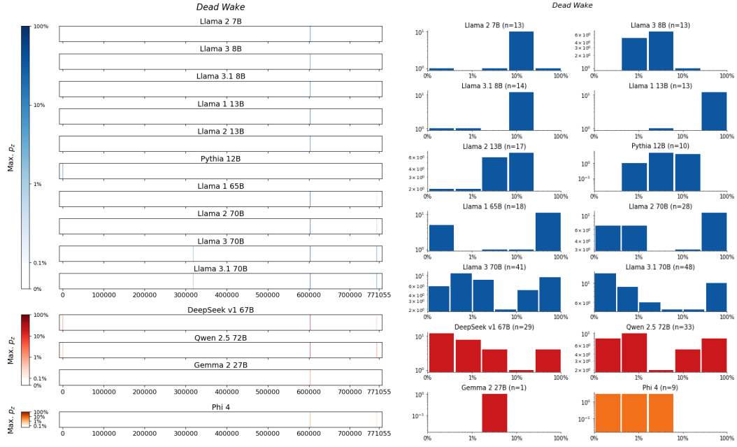
Figure 120: Dead Wake , Larson . For 14 LLMs, (left) heatmaps for the sliding-window procedure and (right) corresponding distributions over suffix extraction probabilities ( \tau_{\min} = 0.1\% ).
