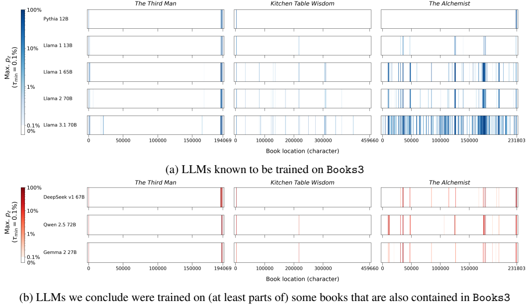
Figure 8: Memorization varies widely across books and models (random books). We apply the sliding-window procedure with top- k decoding ( T=1 , k=40 ) and 100-token sequences (50-token prefixes + 50-token suffixes) for LLMs (a) trained on Books3 (blue) and (b) where it is unknown if Books3 was included in the training data (red). With respect to these settings, LLAMA 3.1 70B memorizes a substantial portion of The Alchemist [52]: extraction coverage is \approx 49.1\% .
