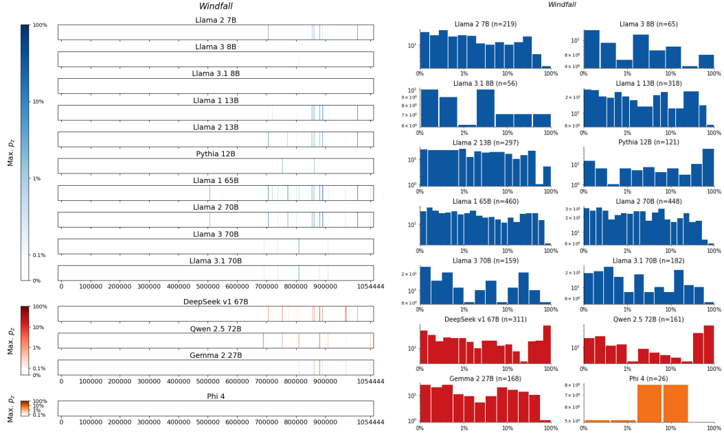
Figure 146: Windfall , O’Sullivan. For 14 LLMs, (left) heatmaps for the sliding-window procedure and (right) corresponding distributions over suffix extraction probabilities ( \tau_{\min} = 0.1\% ).
