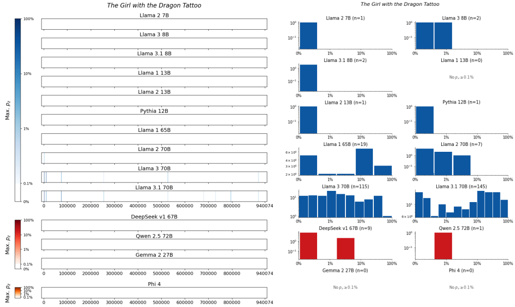
Figure 121: The Girl with the Dragon Tattoo , Larsson . For 14 LLMs, (left) heatmaps for the sliding-window procedure and (right) corresponding distributions over suffix extraction probabilities ( \tau_{\min} = 0.1\% ).
