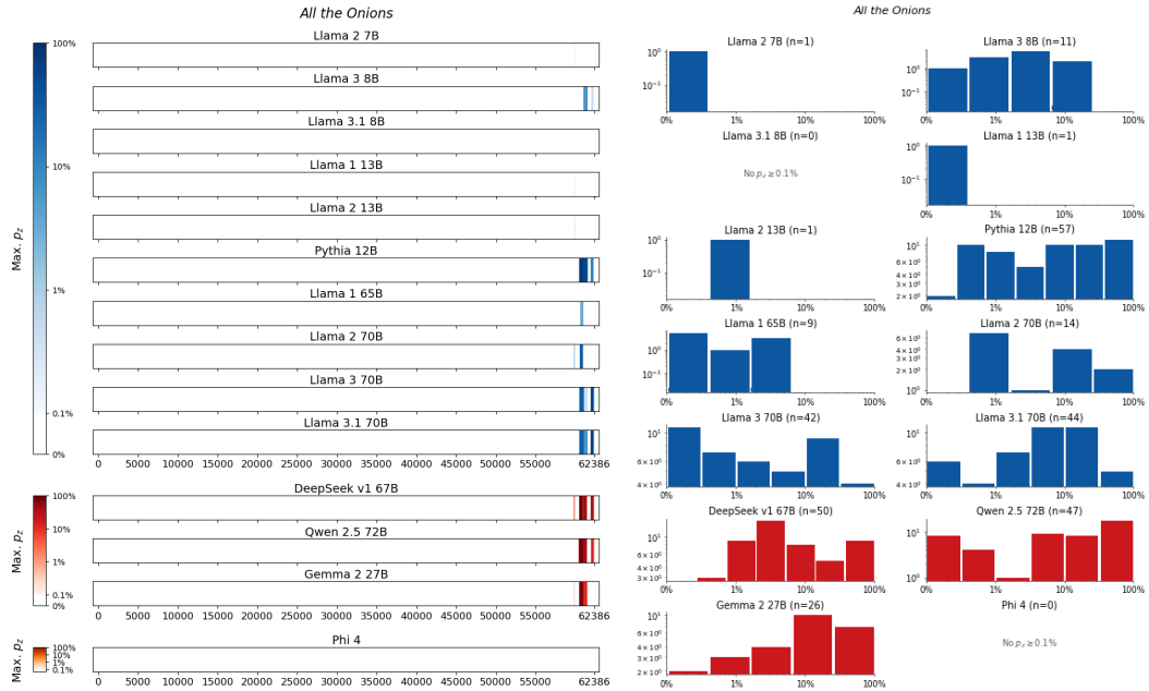
Figure 107: All the Onions, Jacobs . For 14 LLMs, (left) heatmaps for the sliding-window procedure and (right) corresponding distributions over suffix extraction probabilities ( \tau_{\min} = 0.1\% ).
