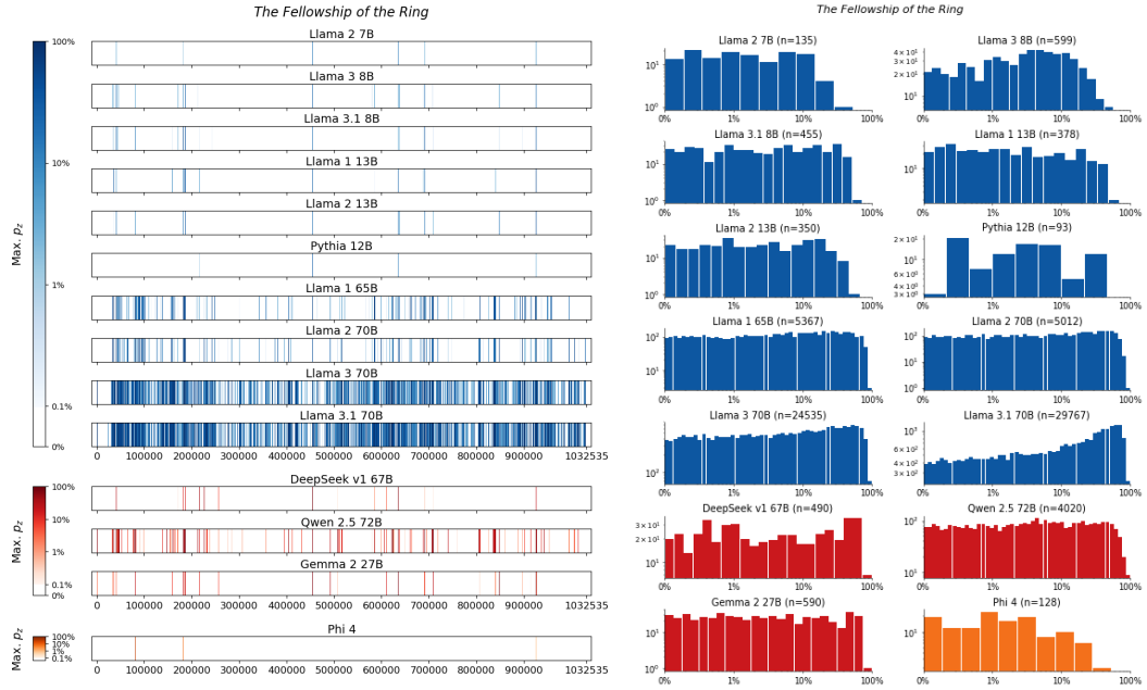
Figure 197: The Fellowship of the Ring , Tolkien. For 14 LLMs, (left) heatmaps for the sliding-window procedure and (right) corresponding distributions over suffix extraction probabilities ( \tau_{\min} = 0.1\% ).
