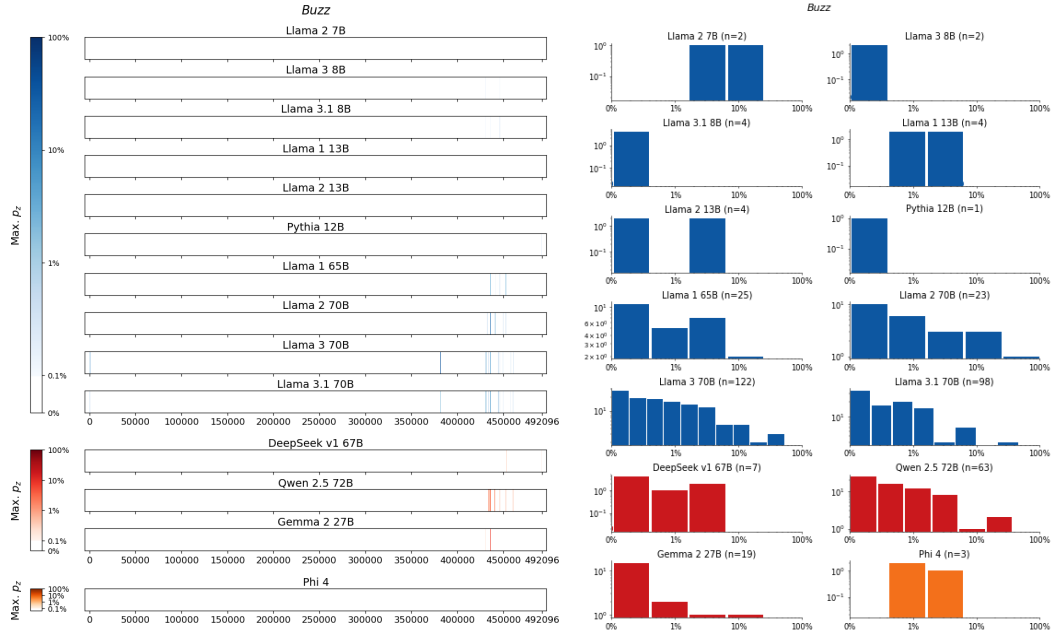
Figure 95: Buzz , Hanson . For 14 LLMs, (left) heatmaps for the sliding-window procedure and (right) corresponding distributions over suffix extraction probabilities ( \tau_{\min} = 0.1\% ).
