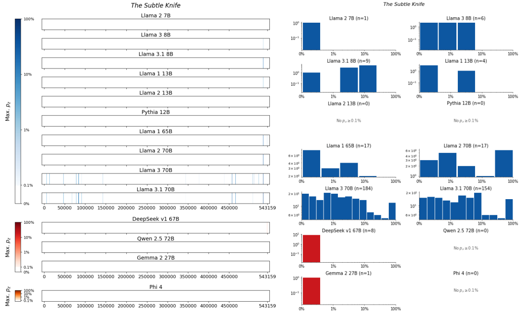
Figure 160: The Subtle Knife , Pullman. For 14 LLMs, (left) heatmaps for the sliding-window procedure and (right) corresponding distributions over suffix extraction probabilities ( \tau_{\min} = 0.1\% ).
