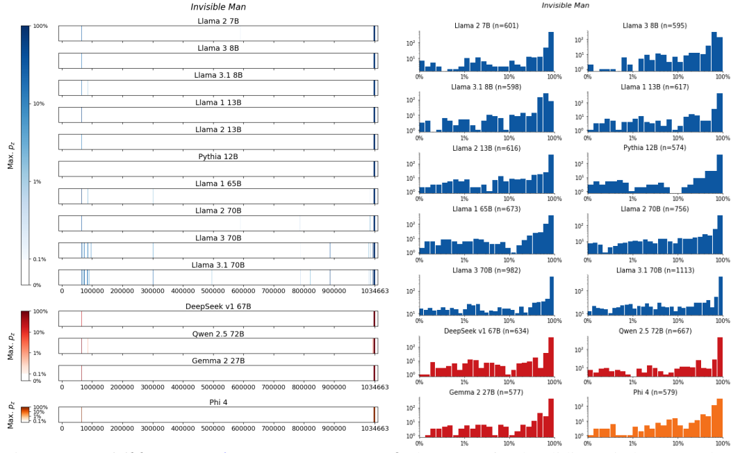
Figure 70: Invisible Man , Ellison. For 14 LLMs, (left) heatmaps for the sliding-window procedure and (right) corresponding distributions over suffix extraction probabilities ( \tau_{\min} = 0.1\% ).
