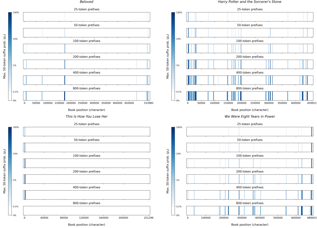
Figure 218: Varying prefix for the LLAMA 2 13B baseline. We run the sliding-window procedure for various prefix lengths for 4 books from Books3: Beloved [187], Harry Potter and the Sorcerer’s Stone [224], This Is How You Lose Her [83], and We Were Eight Years in Power [49]. LLAMA models are known to have been trained on Books3. We run probabilistic extraction on LLAMA 3.1 70B with top- k ( T = 1 , k = 40 ) decoding for 50-token suffixes and prefix lengths in \{25, 50, 100, 200, 400, 800\} . Extraction signal generally increases as prefix length increases. However, this only appears to be the case if there is indeed more memorization to surface; increasing prefix length does not always make previously unextractable sequences extractable. There are also diminishing increases as the prefix lengthens.
