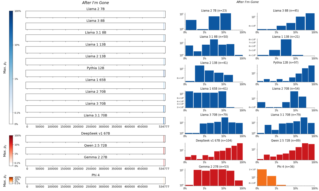
Figure 124: After I'm Gone , Lippman. For 14 LLMs, (left) heatmaps for the sliding-window procedure and (right) corresponding distributions over suffix extraction probabilities ( \tau_{\min} = 0.1\% ).
