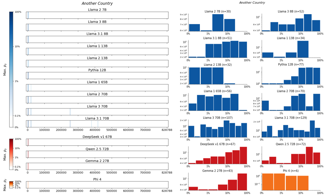
Figure 25: Another Country , Baldwin. For 14 LLMs, (left) heatmaps for the sliding-window procedure and (right) corresponding distributions over suffix extraction probabilities ( \tau_{\min} = 0.1\% ).
