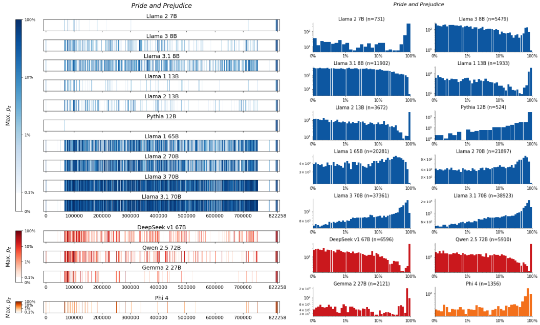
Figure 22: Pride and Prejudice , Austen . For 14 LLMs, (left) heatmaps for the sliding-window procedure and (right) corresponding distributions over suffix extraction probabilities ( \tau_{\min} = 0.1\% ).
