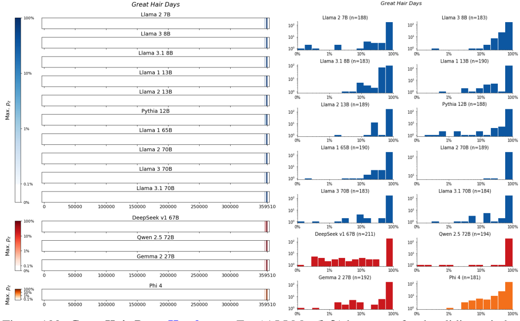
Figure 100: Great Hair Days , Hersheson. For 14 LLMs, (left) heatmaps for the sliding-window procedure and (right) corresponding distributions over suffix extraction probabilities ( \tau_{\min} = 0.1\% ).
