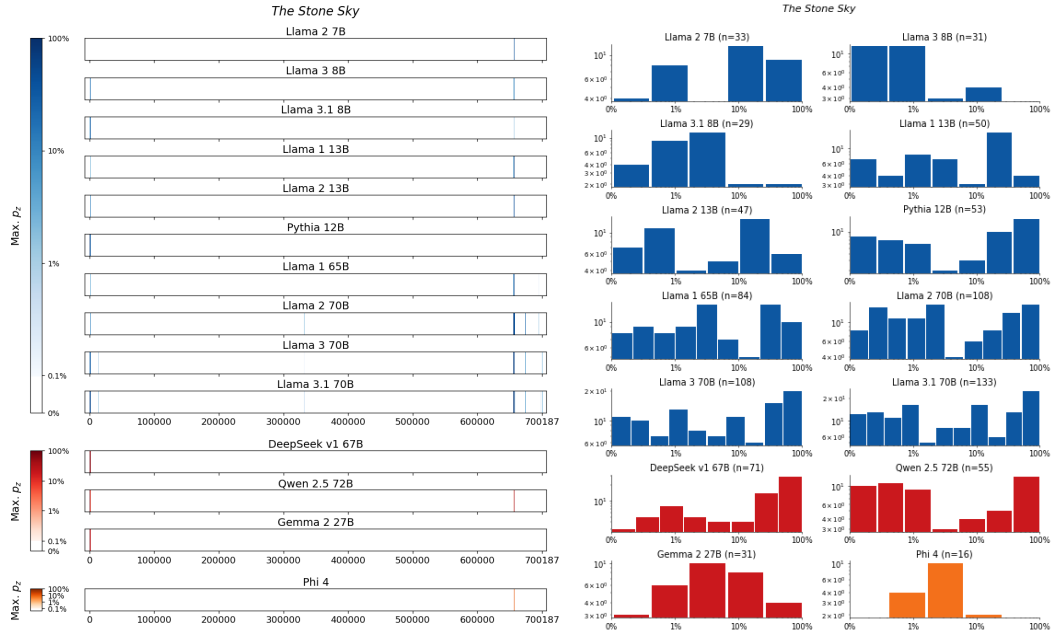
Figure 109: The Stone Sky , Jemisin. For 14 LLMs, (left) heatmaps for the sliding-window procedure and (right) corresponding distributions over suffix extraction probabilities ( \tau_{\min} = 0.1\% ).
