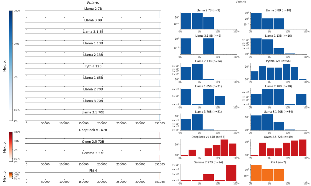
Figure 144: Polaris , Northrop . For 14 LLMs, (left) heatmaps for the sliding-window procedure and (right) corresponding distributions over suffix extraction probabilities ( \tau_{\min} = 0.1\% ).
