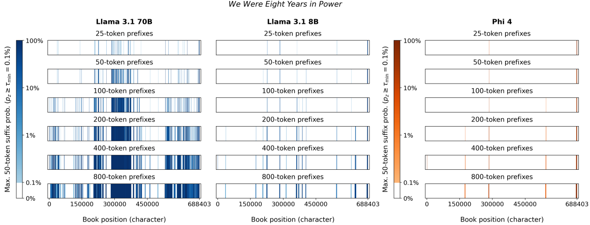
Figure 5: Illustrating validation of our extraction measurements. The sliding-window procedure for LLAMA 3.1 70B, LLAMA 3.1 8B, and PHI 4 on We Were Eight Years in Power [49] (in Books3), using prefix lengths in \{25, 50, 100, 200, 400, 800\} and 50-token suffixes with top- k decoding ( T = 1 , k = 40 ). The book is in LLAMA’s training data, but not PHI 4’s. Longer prefixes reveal more memorized sequences, though not all sequences in the book are extractable as prefix length increases. For PHI 4, the only extractable suffixes are widely duplicated quotes that likely appeared in its training data from other sources. These results support that, when our procedure identifies extraction, it is detecting true instances of memorization rather than chance generations.
