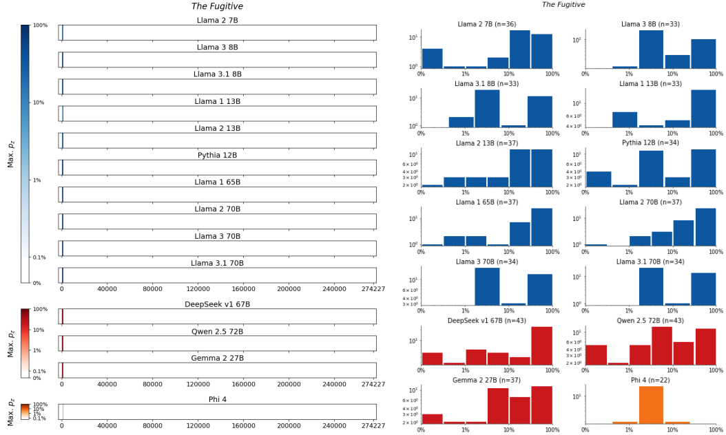
Figure 91: The Fugitive , Grisham. For 14 LLMs, (left) heatmaps for the sliding-window procedure and (right) corresponding distributions over suffix extraction probabilities ( \tau_{\min} = 0.1\% ).
