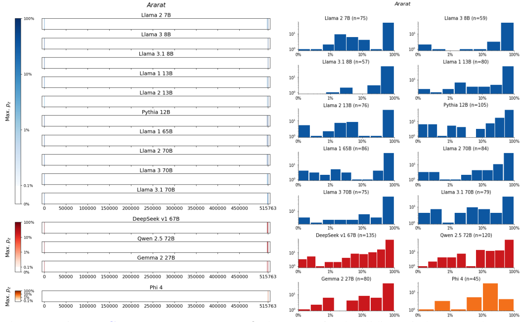
Figure 84: Ararat , Golden . For 14 LLMs, (left) heatmaps for the sliding-window procedure and (right) corresponding distributions over suffix extraction probabilities ( \tau_{\min} = 0.1\% ).
