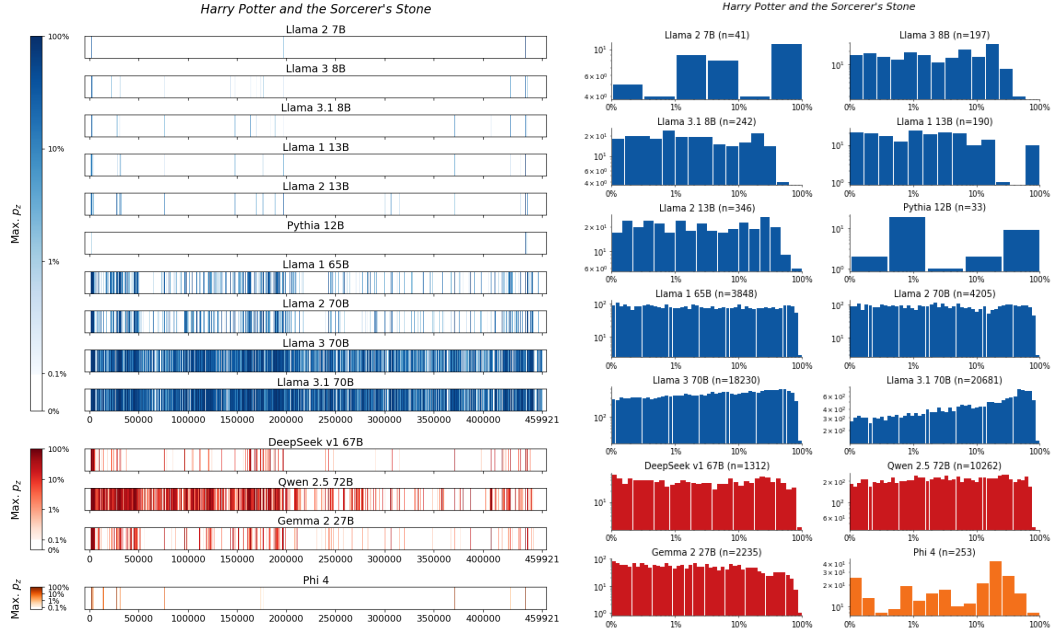
Figure 166: Harry Potter and the Sorcerer's Stone , Rowling. For 14 LLMs, (left) heatmaps for the sliding-window procedure and (right) corresponding distributions over suffix extraction probabilities ( \tau_{\min} = 0.1\% ).
