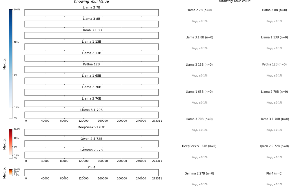
Figure 39: Knowing Your Value , Brzezinski. For 14 LLMs, (left) heatmaps for the sliding-window procedure and (right) corresponding distributions over suffix extraction probabilities ( \tau_{\min} = 0.1\% ).
