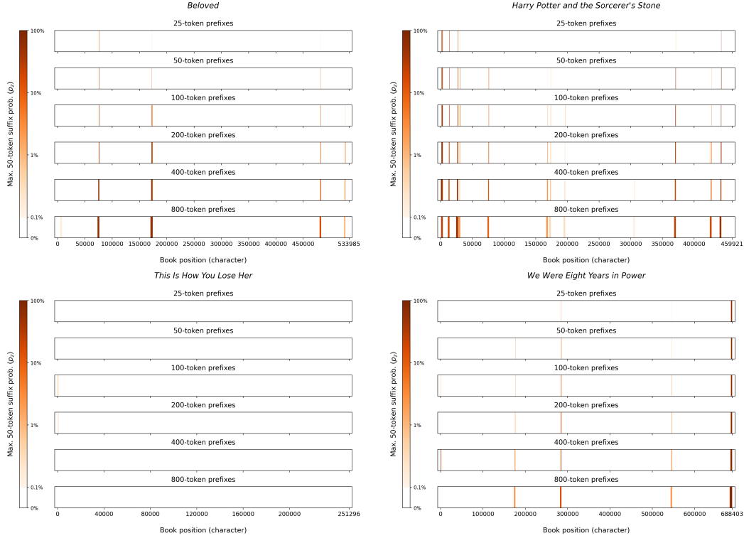
Figure 219: PHI 4 negative controls. Sliding-window procedure for various prefix lengths. We show results for 4 books from Books3: Beloved [187], Harry Potter and the Sorcerer’s Stone [224], This Is How You Lose Her [83], and We Were Eight Years in Power [49]. PHI 4 was deliberately not trained on whole copyrighted books. We run probabilistic extraction on LLAMA 3.1 70B with top- k ( T=1 , k=40 ) decoding for 50-token suffixes and prefix lengths in \{25, 50, 100, 200, 400, 800\} . Extraction signal generally increases as prefix length increases. However, this only appears to be the case if there is indeed more memorization to surface; increasing prefix length does not always make previously unextractable sequences extractable. There are also diminishing increases as the prefix lengthens. We manually verified that every extractable sequence comes from highly duplicated text that can easily be found on the Internet; such sources reasonably were a part of PHI 4’s training data.
