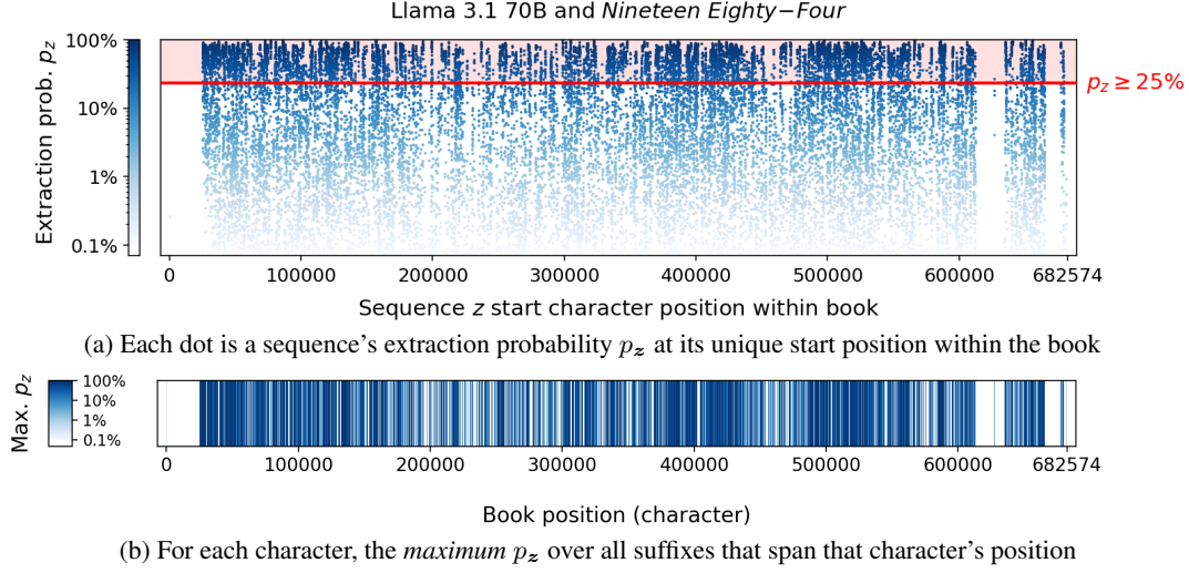
Figure 2: Visualizing our sliding-window probabilistic extraction procedure. For each 100-token window (50-token prefix + 50-token suffix) across 1984 , we compute p_z for LLAMA 3.1 70B with respect to top- k decoding ( T = 1 , k = 40 ). (a) Scatterplot of all extracted sequences z shown by their unique start position in the book. The 100-token sequences overlap significantly. (b) Condensed heatmap view. At each character position, we plot the maximum p_z across all overlapping sequences whose suffixes cover that position. In both plots, colors encode p_z on a log scale. We deem extraction successful if p_z \geq \tau_{\min} = 0.1\% , considering values below this to not reflect extraction (i.e., rounding p_z down to 0%). See Appendix D.
