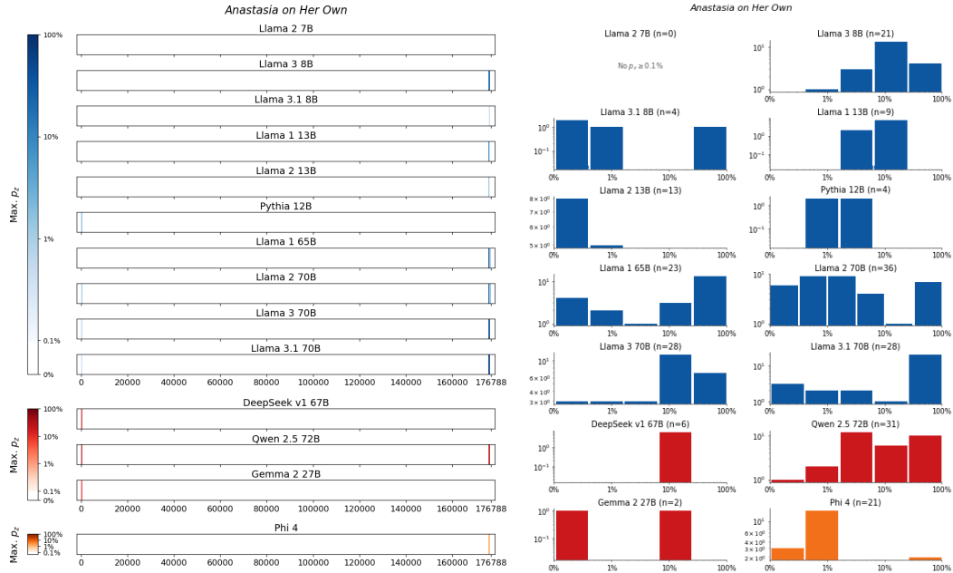
Figure 127: Anastasia on Her Own , Lowry . For 14 LLMs, (left) heatmaps for the sliding-window procedure and (right) corresponding distributions over suffix extraction probabilities ( \tau_{\min} = 0.1\% ).
