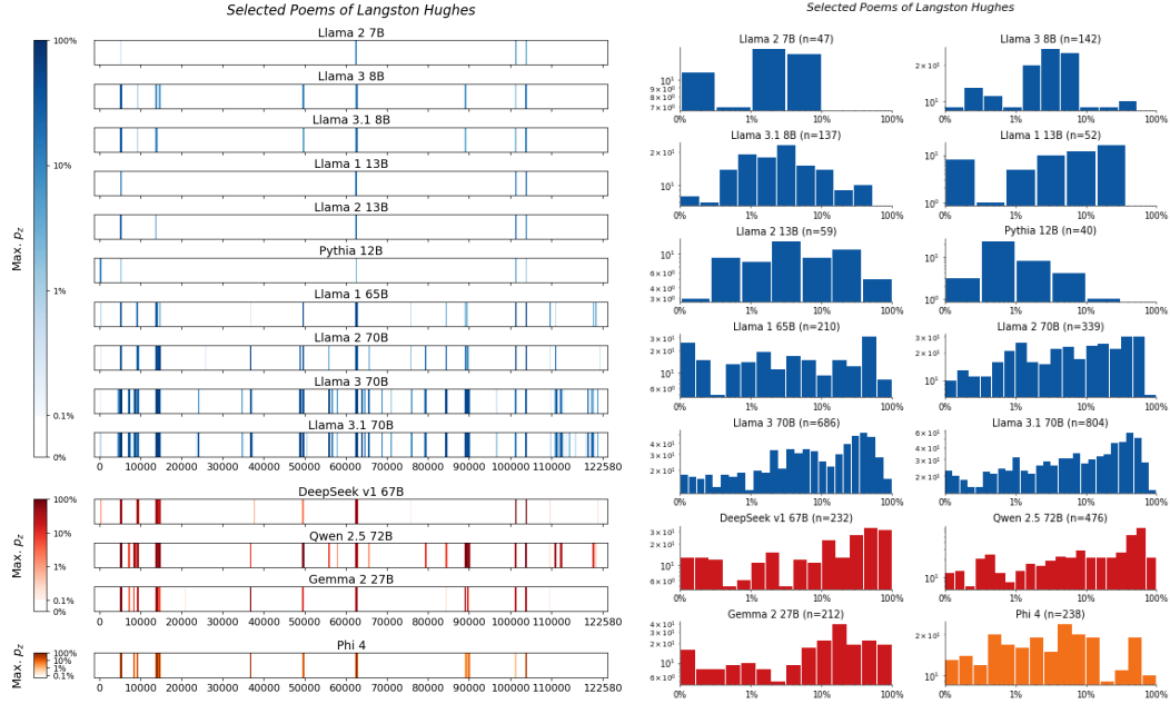
Figure 104: Selected Poems of Langston Hughes , Hughes. For 14 LLMs, (left) heatmaps for the sliding-window procedure and (right) corresponding distributions over suffix extraction probabilities ( \tau_{\min} = 0.1\% ).
