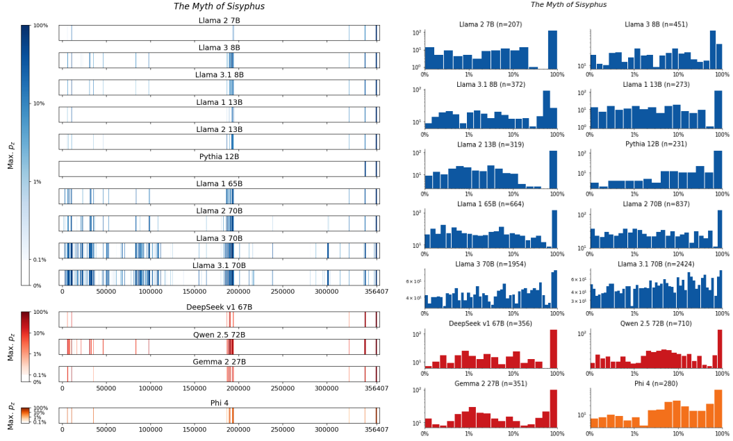
Figure 40: The Myth of Sisyphus , Camus. For 14 LLMs, (left) heatmaps for the sliding-window procedure and (right) corresponding distributions over suffix extraction probabilities ( \tau_{\min} = 0.1\% ).
