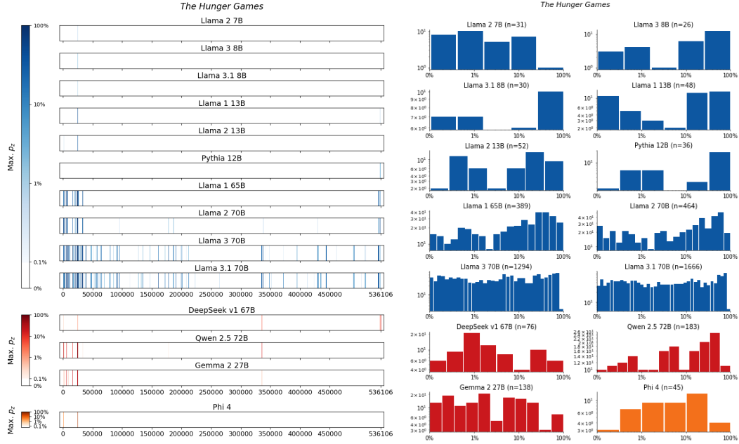
Figure 52: The Hunger Games , Collins. For 14 LLMs, (left) heatmaps for the sliding-window procedure and (right) corresponding distributions over suffix extraction probabilities ( \tau_{\min} = 0.1\% ).
