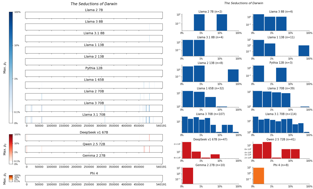
Figure 161: The Seductions of Darwin , Rampley. For 14 LLMs, (left) heatmaps for the sliding-window procedure and (right) corresponding distributions over suffix extraction probabilities ( \tau_{\min} = 0.1\% ).
