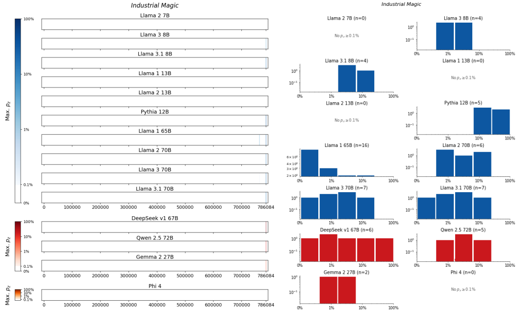
Figure 18: Industrial Magic , Armstrong . For 14 LLMs, (left) heatmaps for the sliding-window procedure and (right) corresponding distributions over suffix extraction probabilities ( \tau_{\min} = 0.1\% ).
