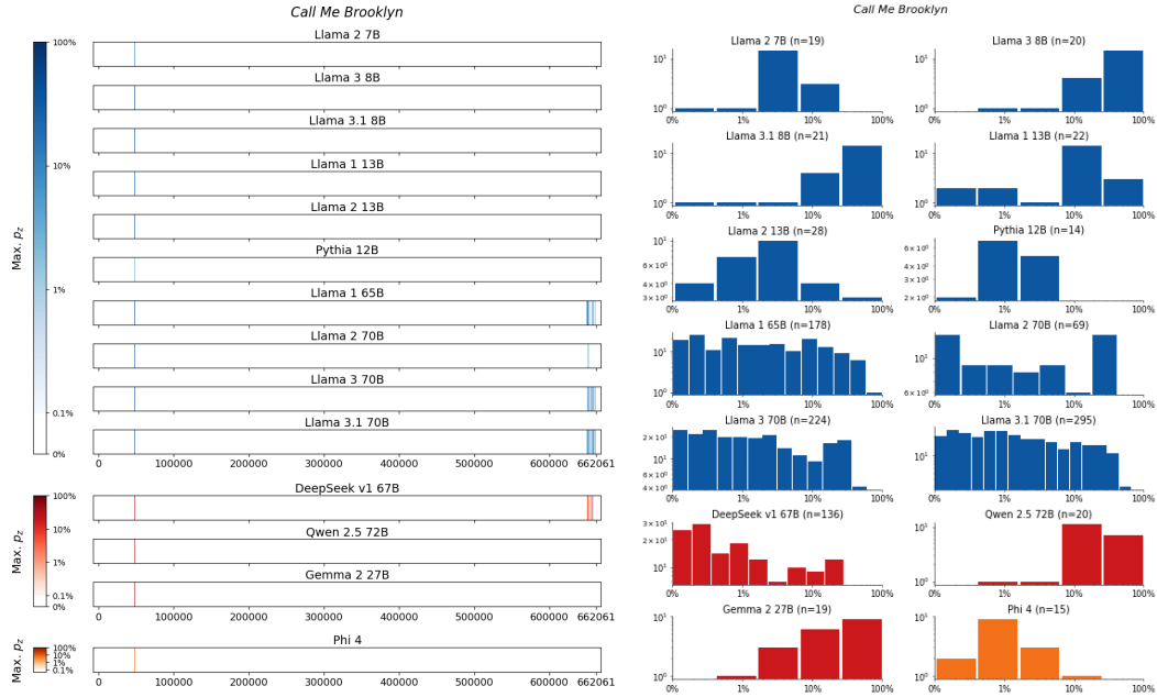
Figure 119: Call Me Brooklyn , Lago. For 14 LLMs, (left) heatmaps for the sliding-window procedure and (right) corresponding distributions over suffix extraction probabilities ( \tau_{\min} = 0.1\% ).
