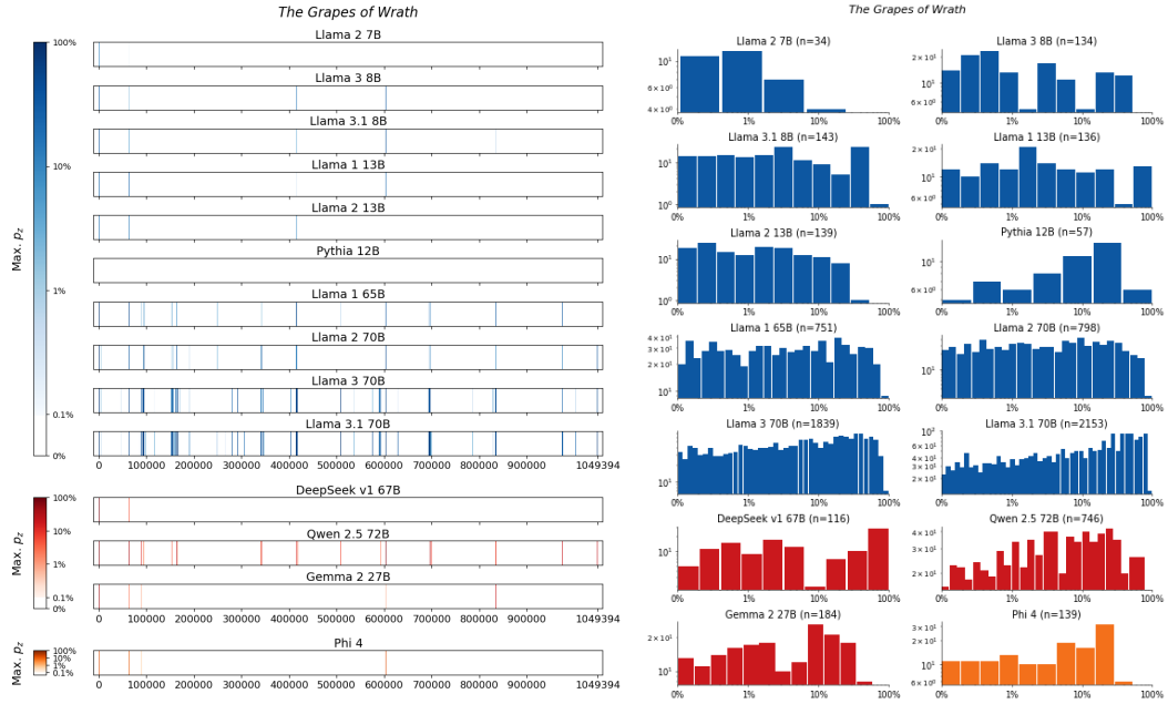
Figure 186: The Grapes of Wrath , Steinbeck. For 14 LLMs, (left) heatmaps for the sliding-window procedure and (right) corresponding distributions over suffix extraction probabilities ( \tau_{\min} = 0.1\% ).
