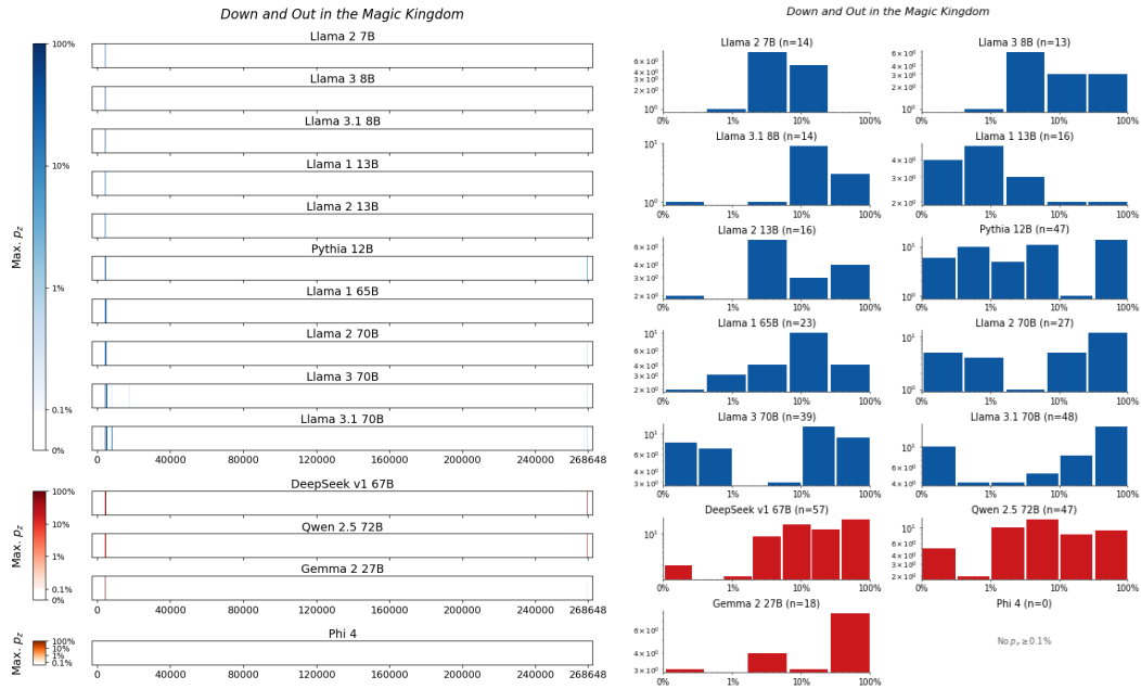
Figure 67: Down and Out in the Magic Kingdom, Doctorow . For 14 LLMs, (left) heatmaps for the sliding-window procedure and (right) corresponding distributions over suffix extraction probabilities ( \tau_{\min} = 0.1\% ).
