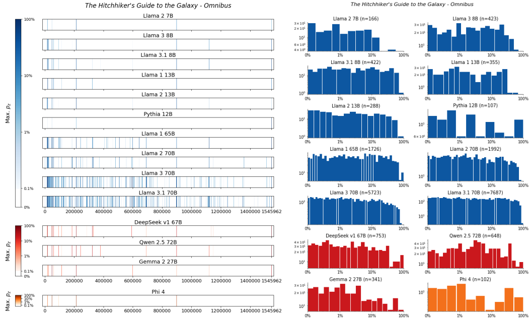
Figure 15: The Hitchhiker's Guide to the Galaxy - Omnibus, Adams . For 14 LLMs, (left) heatmaps for the sliding-window procedure and (right) corresponding distributions over suffix extraction probabilities ( \tau_{\min} = 0.1\% ).
