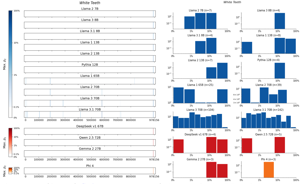
Figure 184: White Teeth , Smith . For 14 LLMs, (left) heatmaps for the sliding-window procedure and (right) corresponding distributions over suffix extraction probabilities ( \tau_{\min} = 0.1\% ).
