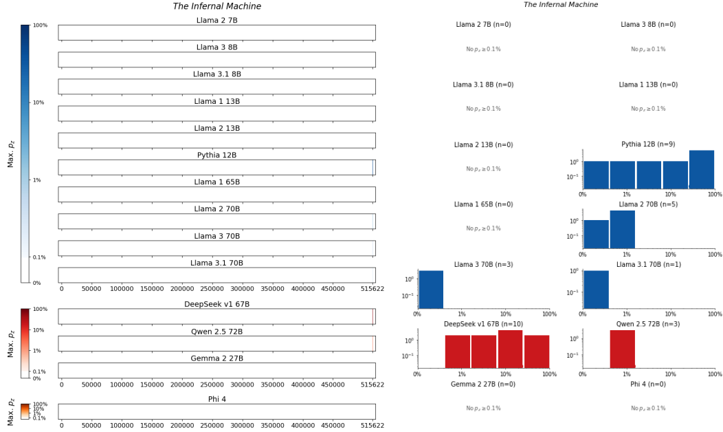
Figure 48: The Infernal Machine, Cocteau . For 14 LLMs, (left) heatmaps for the sliding-window procedure and (right) corresponding distributions over suffix extraction probabilities ( \tau_{\min} = 0.1\% ).
