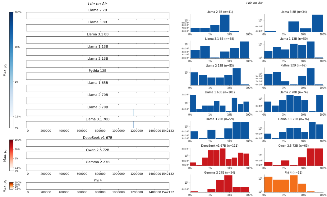
Figure 99: Life on Air , Hendy. For 14 LLMs, (left) heatmaps for the sliding-window procedure and (right) corresponding distributions over suffix extraction probabilities ( \tau_{\min} = 0.1\% ).
