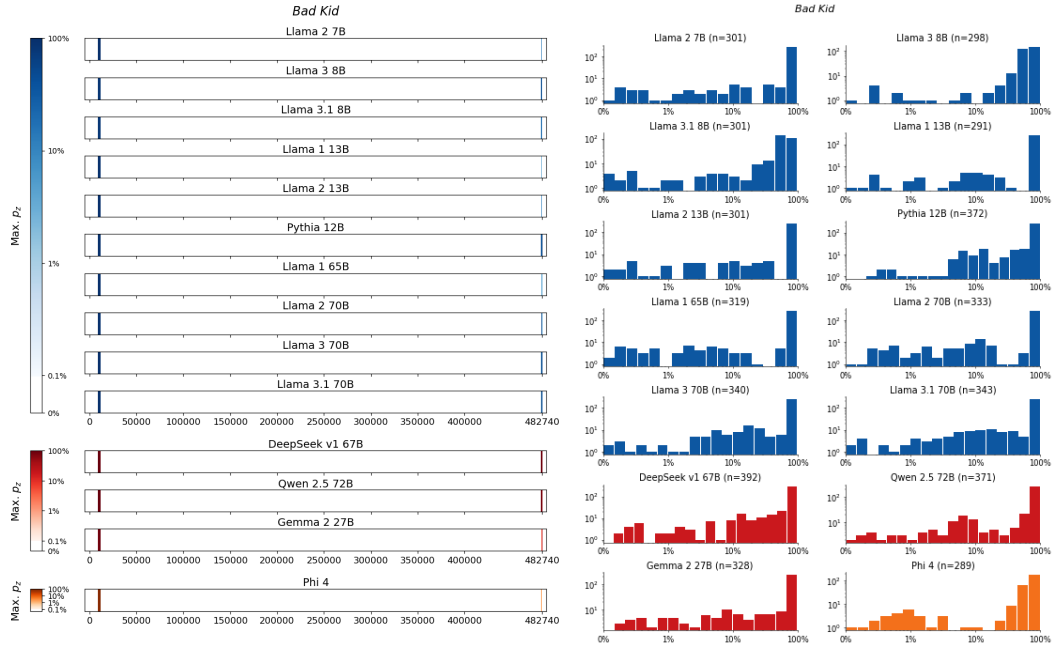
Figure 55: Bad Kid , Crabb. For 14 LLMs, (left) heatmaps for the sliding-window procedure and (right) corresponding distributions over suffix extraction probabilities ( \tau_{\min} = 0.1\% ).
