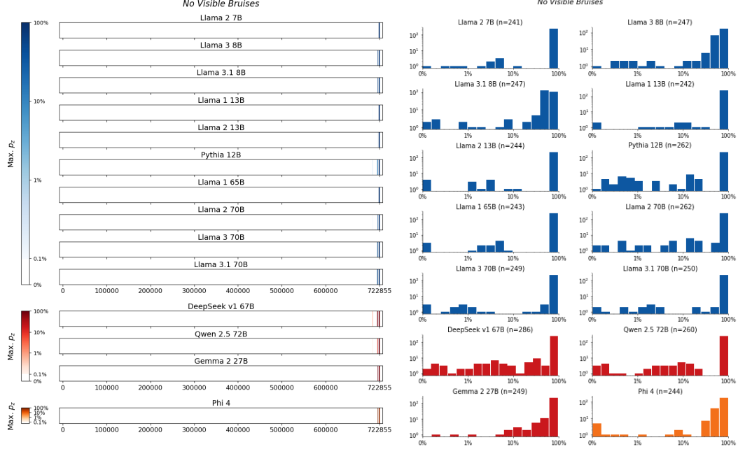
Figure 185: No Visible Bruises , Snyder . For 14 LLMs, (left) heatmaps for the sliding-window procedure and (right) corresponding distributions over suffix extraction probabilities ( \tau_{\min} = 0.1\% ).
