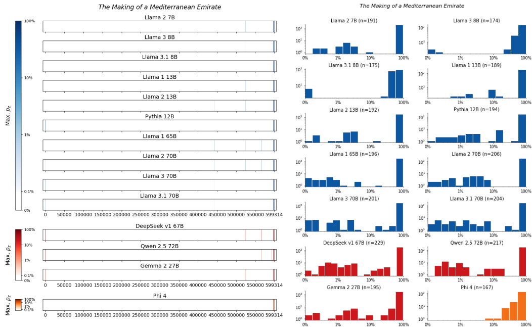
Figure 165: The Making of a Mediterranean Emirate, Roughi . For 14 LLMs, (left) heatmaps for the sliding-window procedure and (right) corresponding distributions over suffix extraction probabilities ( \tau_{\min} = 0.1\% ).
