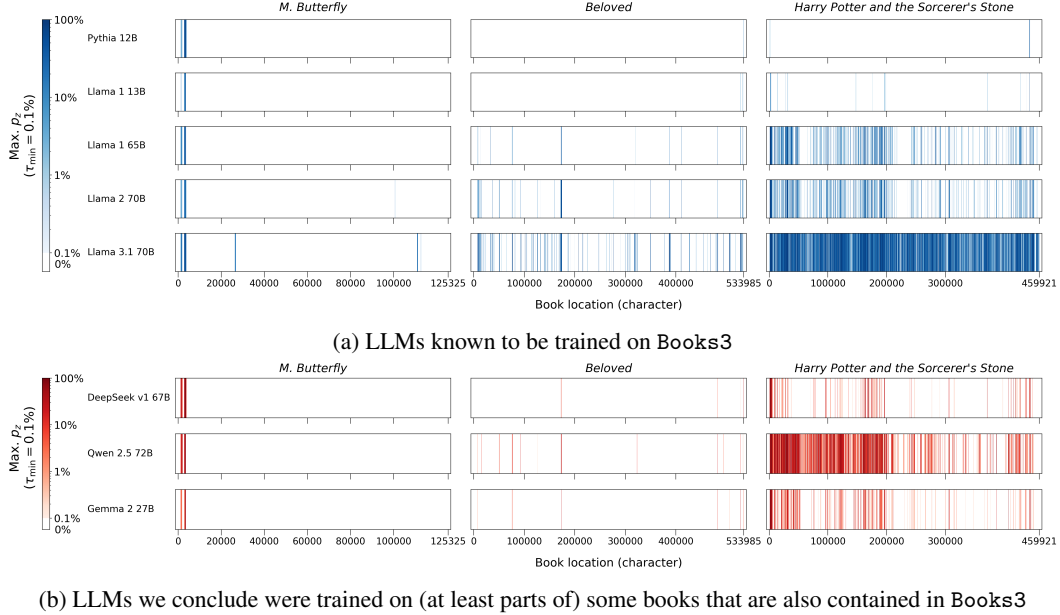
Figure 7: Memorization varies widely across books and models (non-random books). We apply the sliding-window procedure with top- k decoding ( T=1 , k=40 ) and 100-token sequences (50-token prefixes + 50-token suffixes) for LLMs (a) trained on Books3 (blue) and (b) where it is unknown if Books3 was included in the training data (red). With respect to these settings, LLAMA 3.1 70B memorizes effectively all of Harry Potter and the Sorcerer’s Stone [224]: extraction coverage is \approx 96.3\% .
