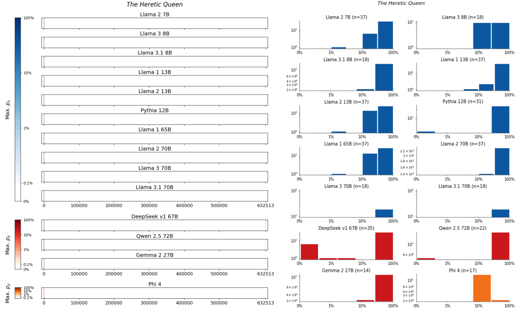
Figure 138: The Heretic Queen , Moran . For 14 LLMs, (left) heatmaps for the sliding-window procedure and (right) corresponding distributions over suffix extraction probabilities ( \tau_{\min} = 0.1\% ).
