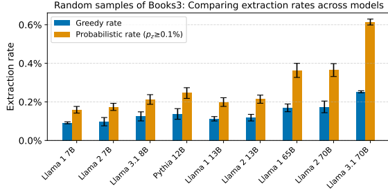
Figure 3: Average extraction rates are low, but book-specific extraction varies widely. (left) Comparing extraction rates (Equation 3) of random 100-token sequences (50-token prefix + 50-token suffix) from Books3 for different LLMs trained on Books3. Average extraction is low (Appendix C) for both greedy discoverable and probabilistic ( p_z \geq \tau_{\min} = 0.1\% , top- k with T = 1 and k = 40 ) extraction. (right) Extraction coverage (Equation 4) for specific books reveals a more nuanced picture. For Harry Potter [224] and Sandman Slim [142], we show extraction coverage for \tau \in \{1\%, 10\%, 50\%\} for 3 models (Appendix D.4). Nearly half of Harry Potter can be extracted with respect to sequences that exhibit p_z \geq \tau = 50\% .
