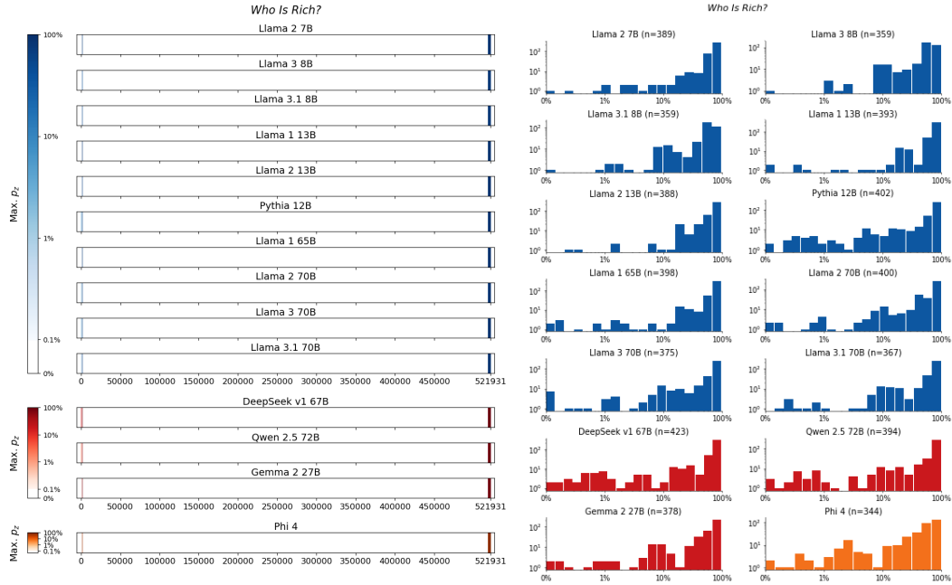
Figure 113: Who Is Rich? , Klam. For 14 LLMs, (left) heatmaps for the sliding-window procedure and (right) corresponding distributions over suffix extraction probabilities ( \tau_{\min} = 0.1\% ).
