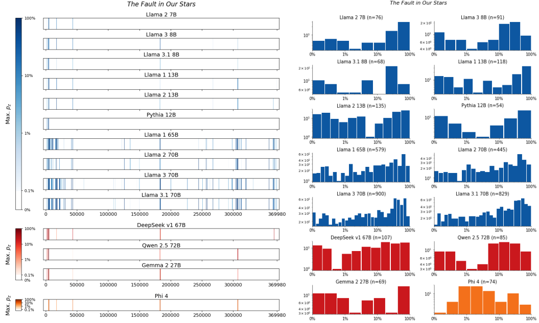
Figure 88: The Fault in Our Stars , Green . For 14 LLMs, (left) heatmaps for the sliding-window procedure and (right) corresponding distributions over suffix extraction probabilities ( \tau_{\min} = 0.1\% ).
