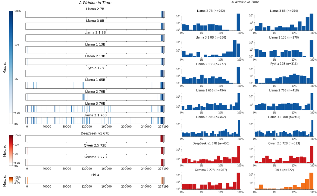
Figure 118: A Wrinkle in Time , L'Engle. For 14 LLMs, (left) heatmaps for the sliding-window procedure and (right) corresponding distributions over suffix extraction probabilities ( \tau_{\min} = 0.1\% ).
