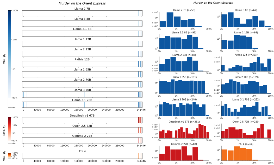
Figure 43: Murder on the Orient Express , Christie . For 14 LLMs, (left) heatmaps for the sliding-window procedure and (right) corresponding distributions over suffix extraction probabilities ( \tau_{\min} = 0.1\% ).
