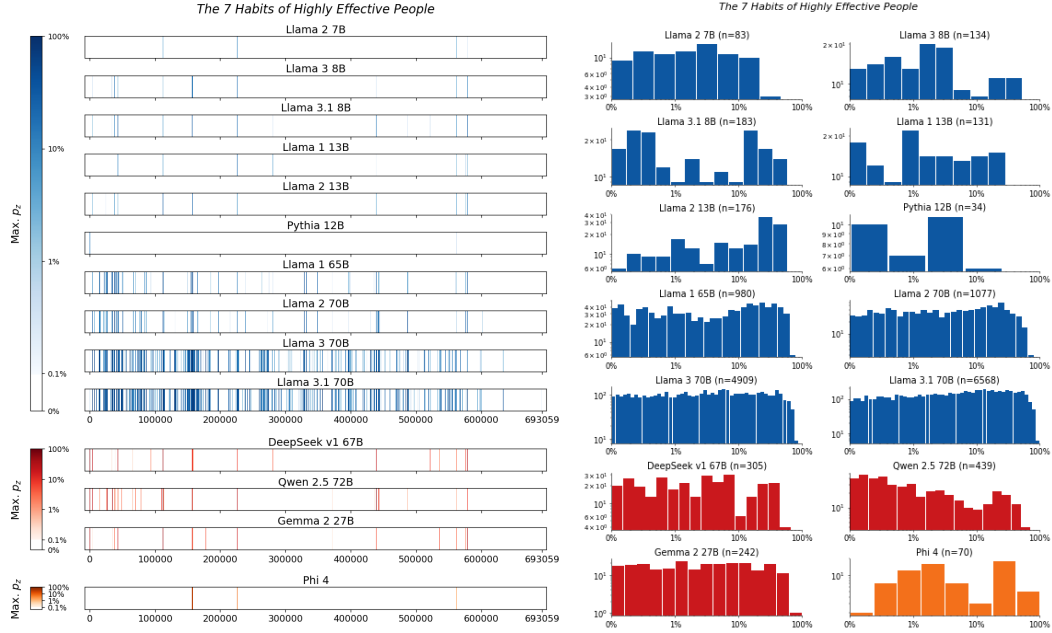
Figure 54: The 7 Habits of Highly Effective People , Covey. For 14 LLMs, (left) heatmaps for the sliding-window procedure and (right) corresponding distributions over suffix extraction probabilities ( \tau_{\min} = 0.1\% ).
