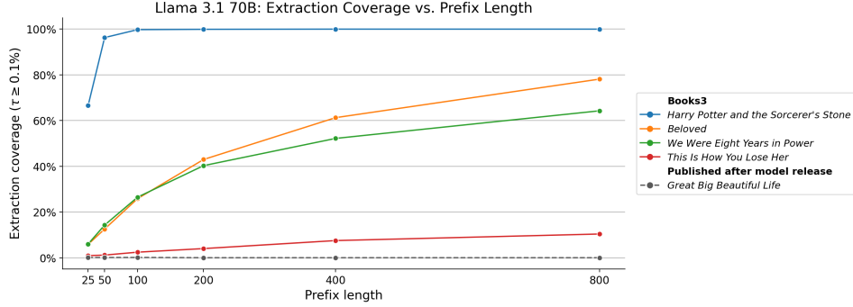
Figure 6: Extraction coverage by prefix length. Plotting extraction coverage for \tau = \tau_{\min} = 0.1\% (Equation 4) for 5 books we test with varying prefix lengths and LLAMA 3.1 70B. 4 of these books are in Books3 and thus in LLAMA’s training data. The remaining book, Great Big Beautiful Life [128], is used in our negative controls on non-training data; extraction coverage is 0% (aside from the copyright notice) regardless of prefix length. As we increase prefix length, extraction coverage for each book in the training data begins to level off. While Harry Potter [224] is entirely memorized, it does not appear to be the case that Beloved [187], We Were Eight Years in Power [49], or This Is How You Lose Her [83] are entirely extractable with respect to 50-token suffixes and even longer prefixes.
