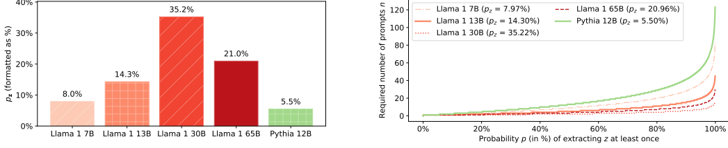
Figure 11: Plotting p_z for the “careless people” quote from The Great Gatsby . (left) p_z (1) for different models. (right) Translating p_z into how many prompts n it would take to extract the sequence z with at least probability p (5). See Section 2.
