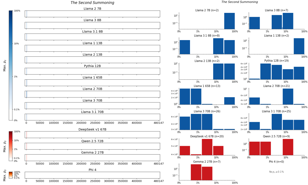
Figure 103: The Second Summoning , Huff . For 14 LLMs, (left) heatmaps for the sliding-window procedure and (right) corresponding distributions over suffix extraction probabilities ( \tau_{\min} = 0.1\% ).
